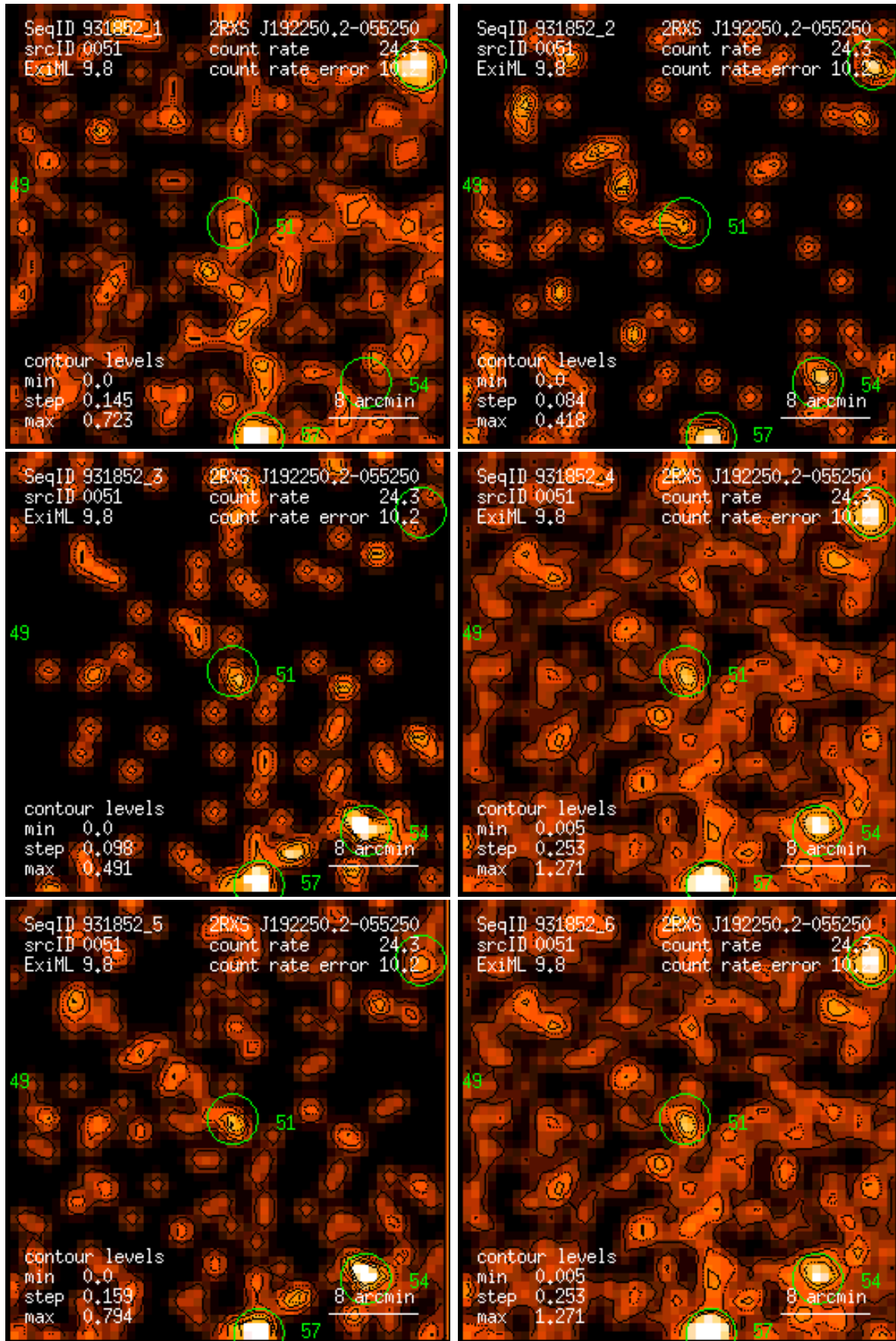
Figure 51: RASS 931852: detection 0051: band rate images, Gaussian filter: (1) PSPC channels 11 – 41, (2) 52 – 90, (3) 91 – 201, (4) 11 – 235, (5) 52 – 201, (6) 11 – 201. Broad band rates in counts/ks. Band rate contour levels in counts/ks/arcmin 2 .
