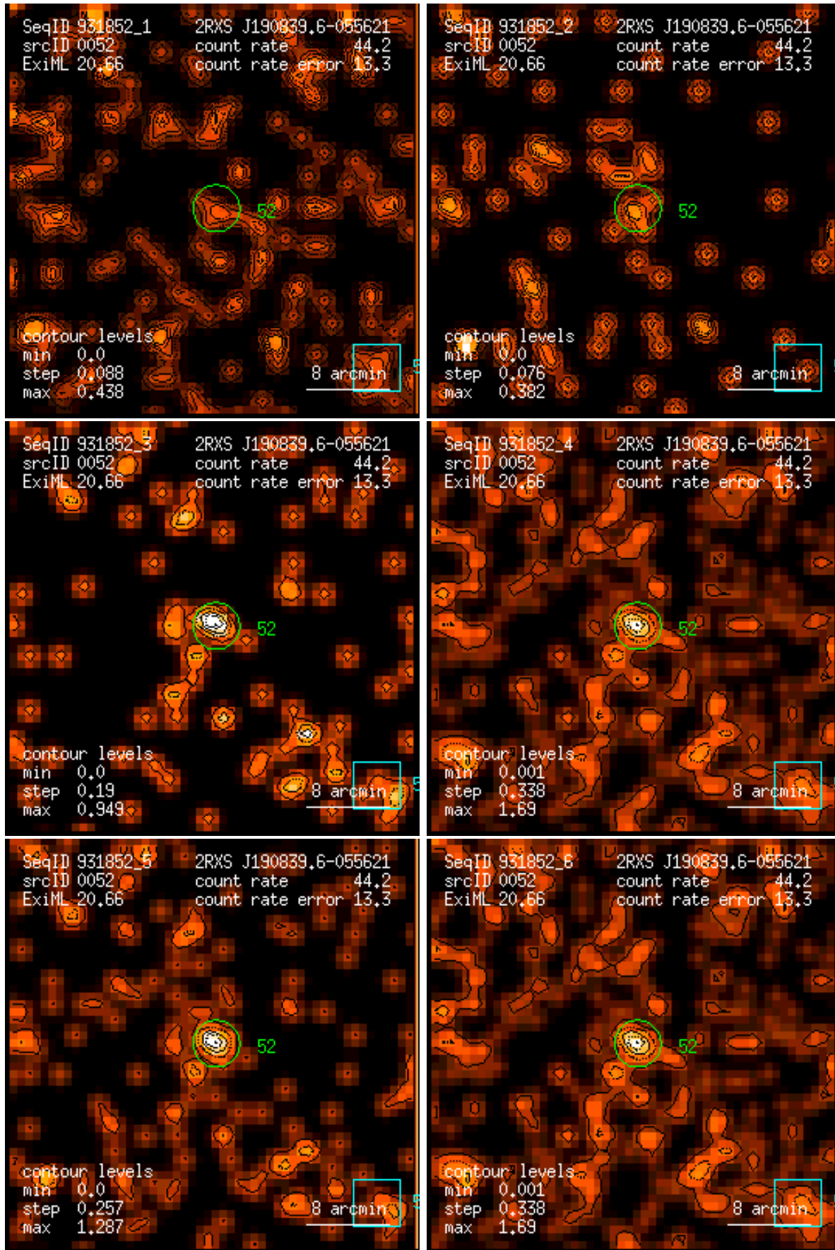
Figure 52: RASS 931852: detection 0052: band rate images, Gaussian filter: (1) PSPC channels 11 – 41, (2) 52 – 90, (3) 91 – 201, (4) 11 – 235, (5) 52 – 201, (6) 11 – 201. Broad band rates in counts/ks. Band rate contour levels in counts/ks/arcmin 2 .
