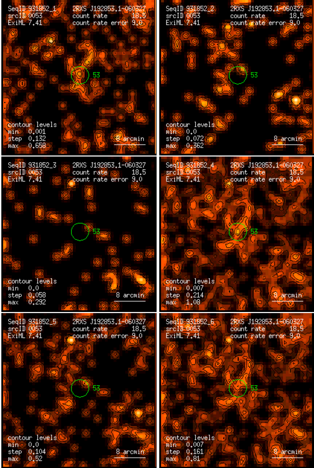
Figure 53: RASS 931852: detection 0053: band rate images, Gaussian filter: (1) PSPC channels 11 – 41, (2) 52 – 90, (3) 91 – 201, (4) 11 – 235, (5) 52 – 201, (6) 11 – 201. Broad band rates in counts/ks. Band rate contour levels in counts/ks/arcmin 2 .
