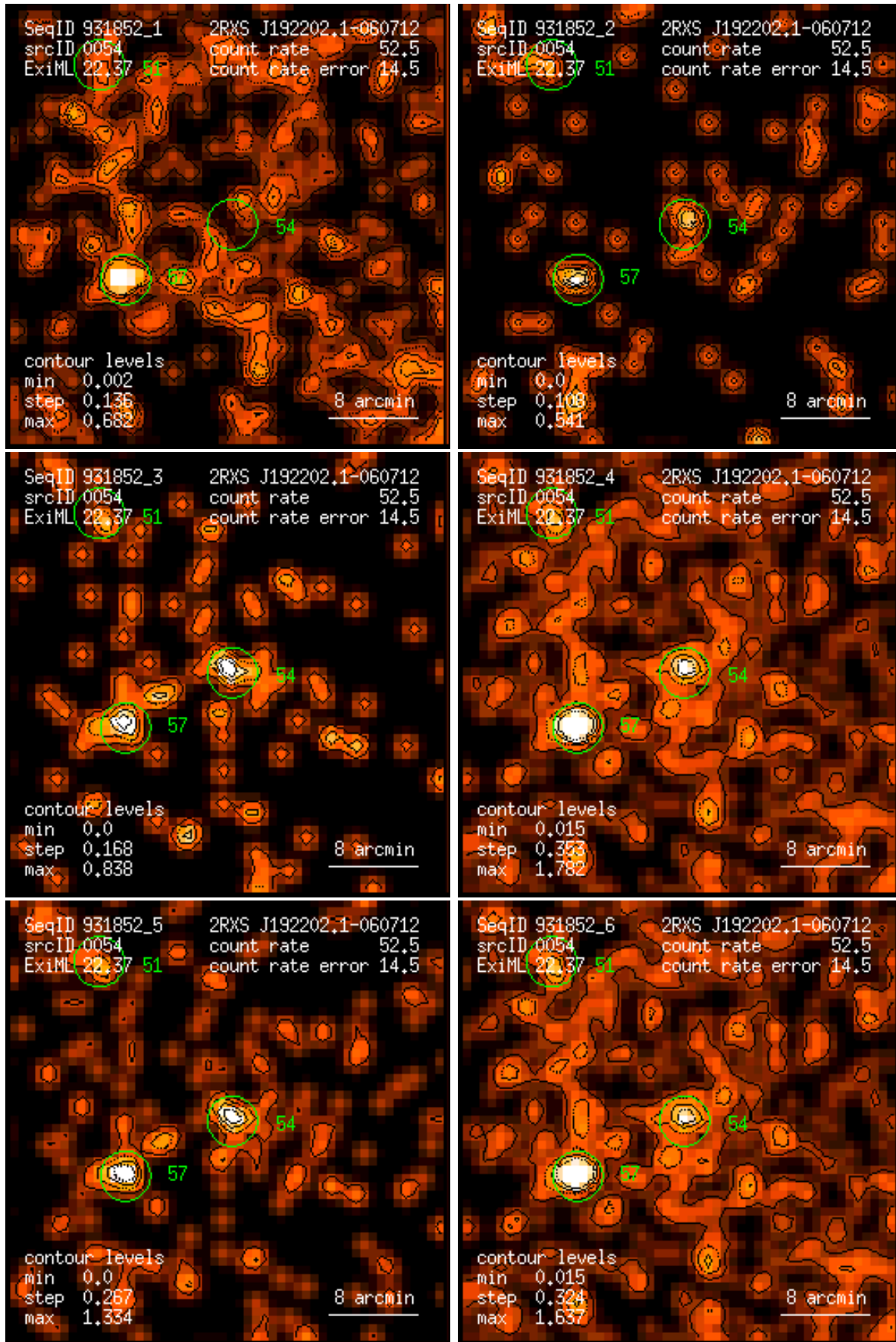
Figure 54: RASS 931852: detection 0054: band rate images, Gaussian filter: (1) PSPP channels 11 – 41, (2) 52 – 90, (3) 91 – 201, (4) 11 – 235, (5) 52 – 201, (6) 11 – 201. Broad band rates in counts/ks. Band rate contour levels in counts/ks/arcmin 2 .
