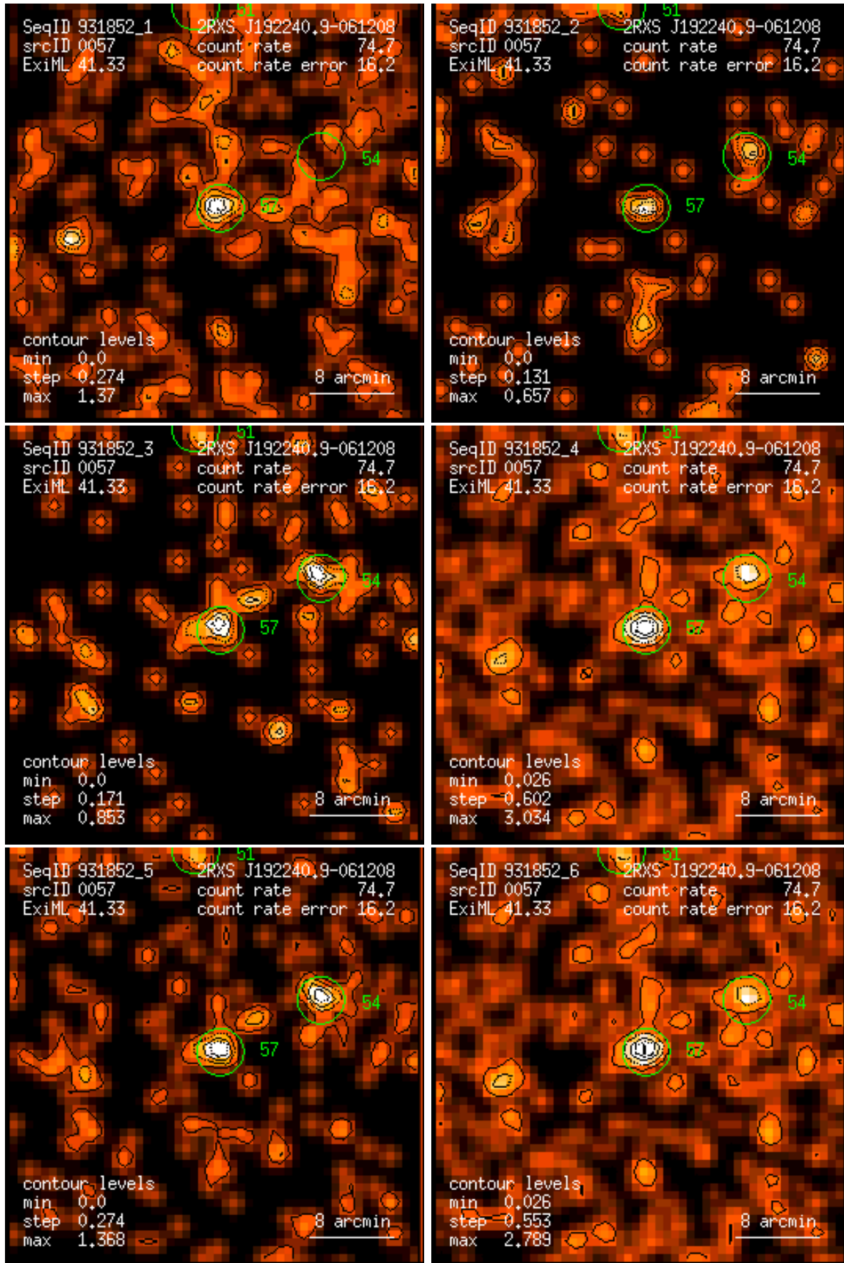
Figure 57: RASS 931852: detection 0057: band rate images, Gaussian filter: (1) PSPC channels 11 – 41, (2) 52 – 90, (3) 91 – 201, (4) 11 – 235, (5) 52 – 201, (6) 11 – 201. Broad band rates in counts/ks. Band rate contour levels in counts/ks/arcmin 2 .
