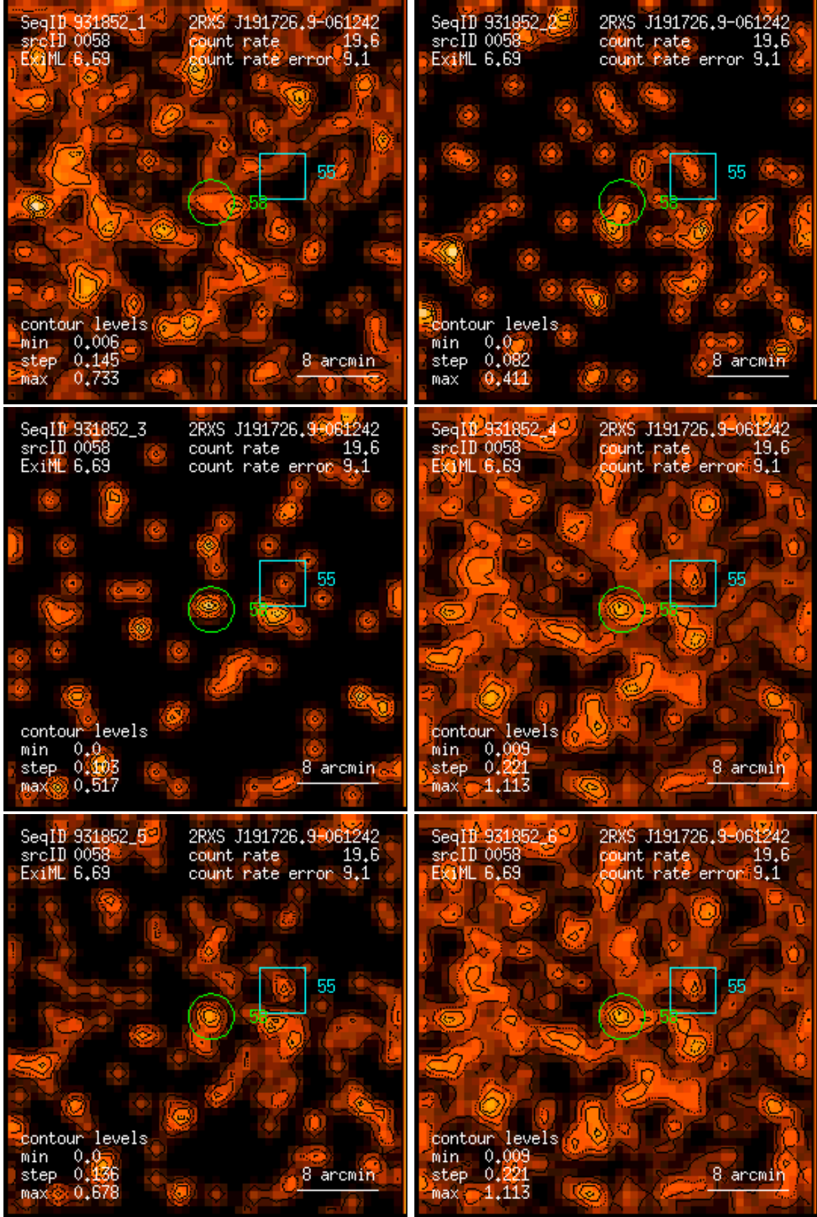
Figure 58: RASS 931852: detection 0058: band rate images, Gaussian filter: (1) PSPC channels 11 – 41, (2) 52 – 90, (3) 91 – 201, (4) 11 – 235, (5) 52 – 201, (6) 11 – 201. Broad band rates in counts/ks. Band rate contour levels in counts/ks/arcmin 2 .
