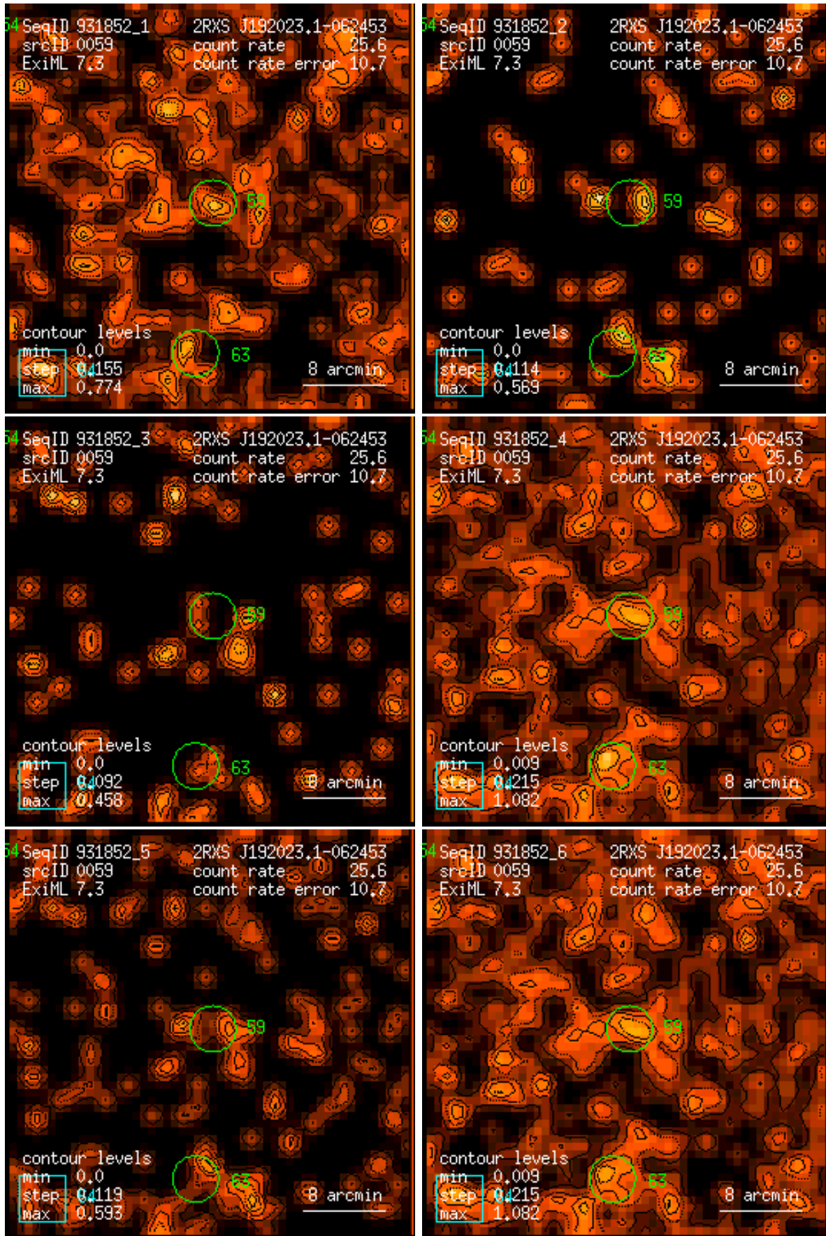
Figure 59: RASS 931852: detection 0059: band rate images, Gaussian filter: (1) PSPC channels 11 – 41, (2) 52 – 90, (3) 91 – 201, (4) 11 – 235, (5) 52 – 201, (6) 11 – 201. Broad band rates in counts/ks. Band rate contour levels in counts/ks/arcmin 2 .
