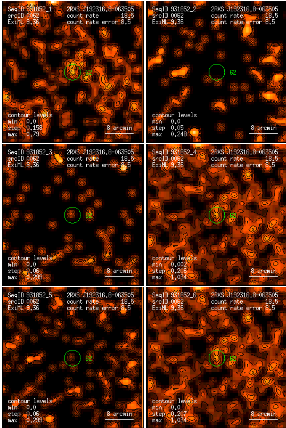
Figure 62: RASS 931852: detection 0062: band rate images, Gaussian filter: (1) PSPC channels 11 – 41, (2) 52 – 90, (3) 91 – 201, (4) 11 – 235, (5) 52 – 201, (6) 11 – 201. Broad band rates in counts/ks. Band rate contour levels in counts/ks/arcmin 2 .
