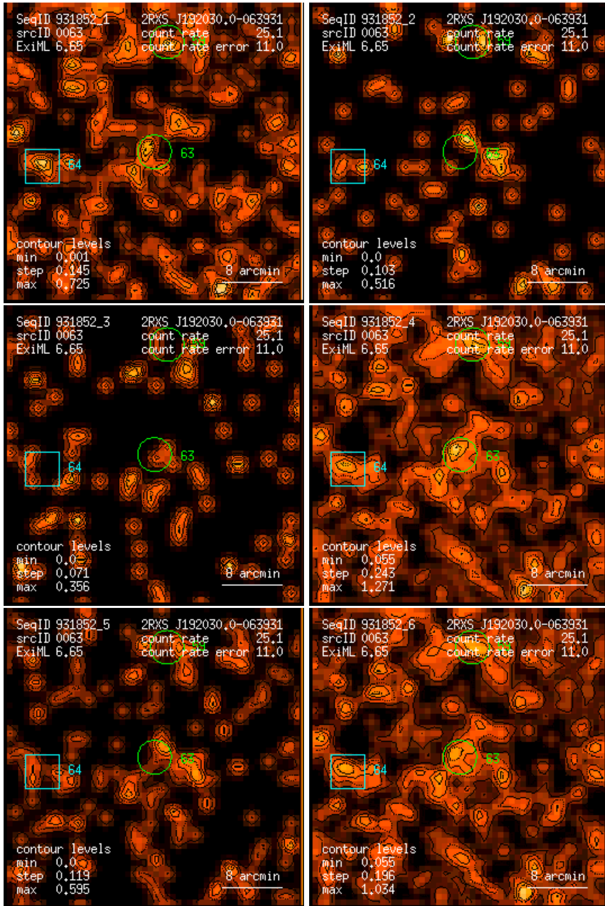
Figure 63: RASS 931852: detection 0063: band rate images, Gaussian filter: (1) PSPC channels 11 – 41, (2) 52 – 90, (3) 91 – 201, (4) 11 – 235, (5) 52 – 201, (6) 11 – 201. Broad band rates in counts/ks. Band rate contour levels in counts/ks/arcmin 2 .
