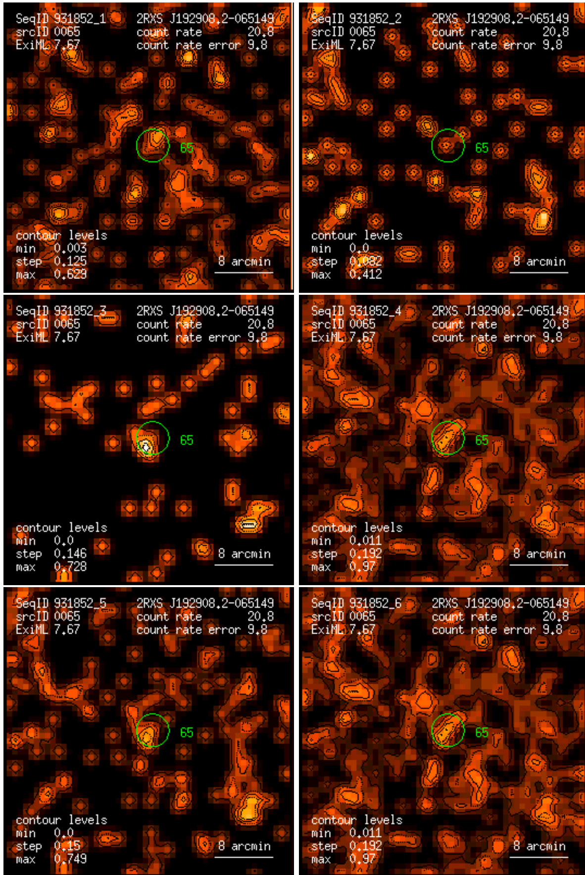
Figure 65: RASS 931852: detection 0065: band rate images, Gaussian filter: (1) PSPC channels 11 – 41, (2) 52 – 90, (3) 91 – 201, (4) 11 – 235, (5) 52 – 201, (6) 11 – 201. Broad band rates in counts/ks. Band rate contour levels in counts/ks/arcmin 2 .
