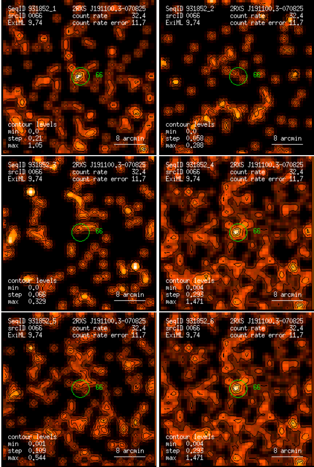
Figure 66: RASS 931852: detection 0066: band rate images, Gaussian filter: (1) PSPC channels 11 – 41, (2) 52 – 90, (3) 91 – 201, (4) 11 – 235, (5) 52 – 201, (6) 11 – 201. Broad band rates in counts/ks. Band rate contour levels in counts/ks/arcmin 2 .
