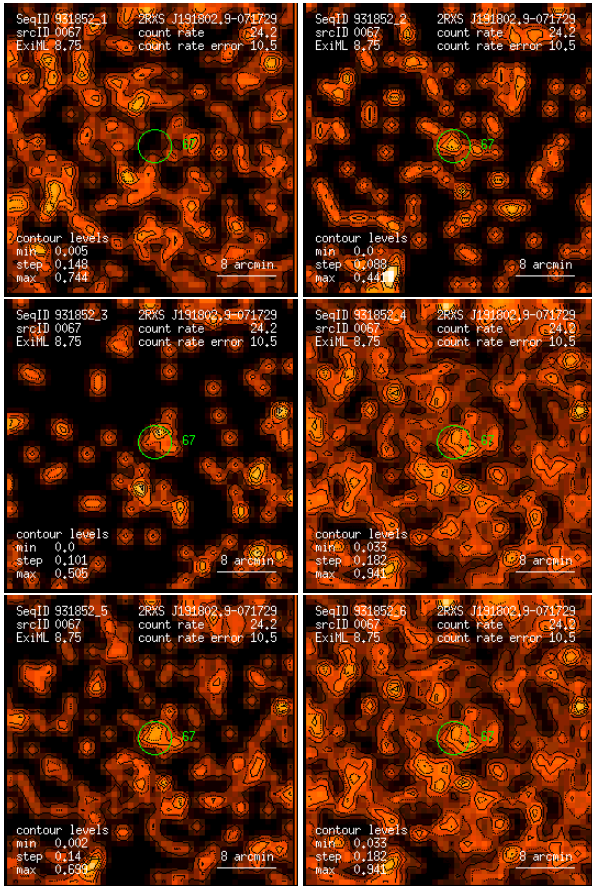
Figure 67: RASS 931852: detection 0067: band rate images, Gaussian filter: (1) PSPC channels 11 – 41, (2) 52 – 90, (3) 91 – 201, (4) 11 – 235, (5) 52 – 201, (6) 11 – 201. Broad band rates in counts/ks. Band rate contour levels in counts/ks/arcmin 2 .
