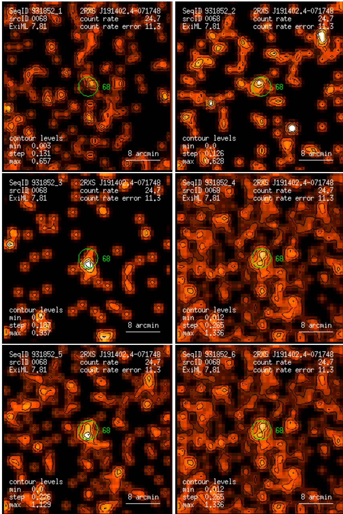
Figure 68: RASS 931852: detection 0068: band rate images, Gaussian filter: (1) PSPC channels 11 – 41, (2) 52 – 90, (3) 91 – 201, (4) 11 – 235, (5) 52 – 201, (6) 11 – 201. Broad band rates in counts/ks. Band rate contour levels in counts/ks/arcmin 2 .
