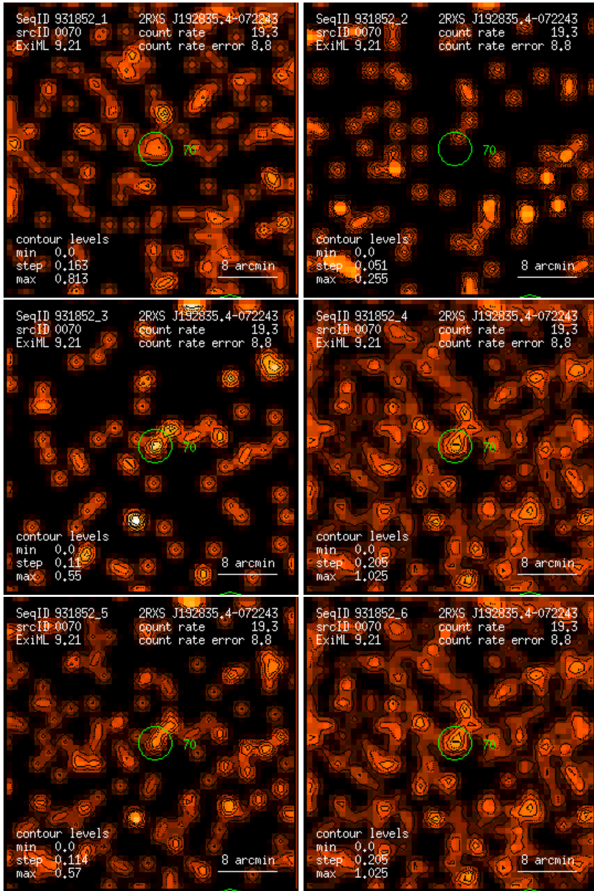
Figure 70: RASS 931852: detection 0070: band rate images, Gaussian filter: (1) PSPC channels 11 – 41, (2) 52 – 90, (3) 91 – 201, (4) 11 – 235, (5) 52 – 201, (6) 11 – 201. Broad band rates in counts/ks. Band rate contour levels in counts/ks/arcmin 2 .
