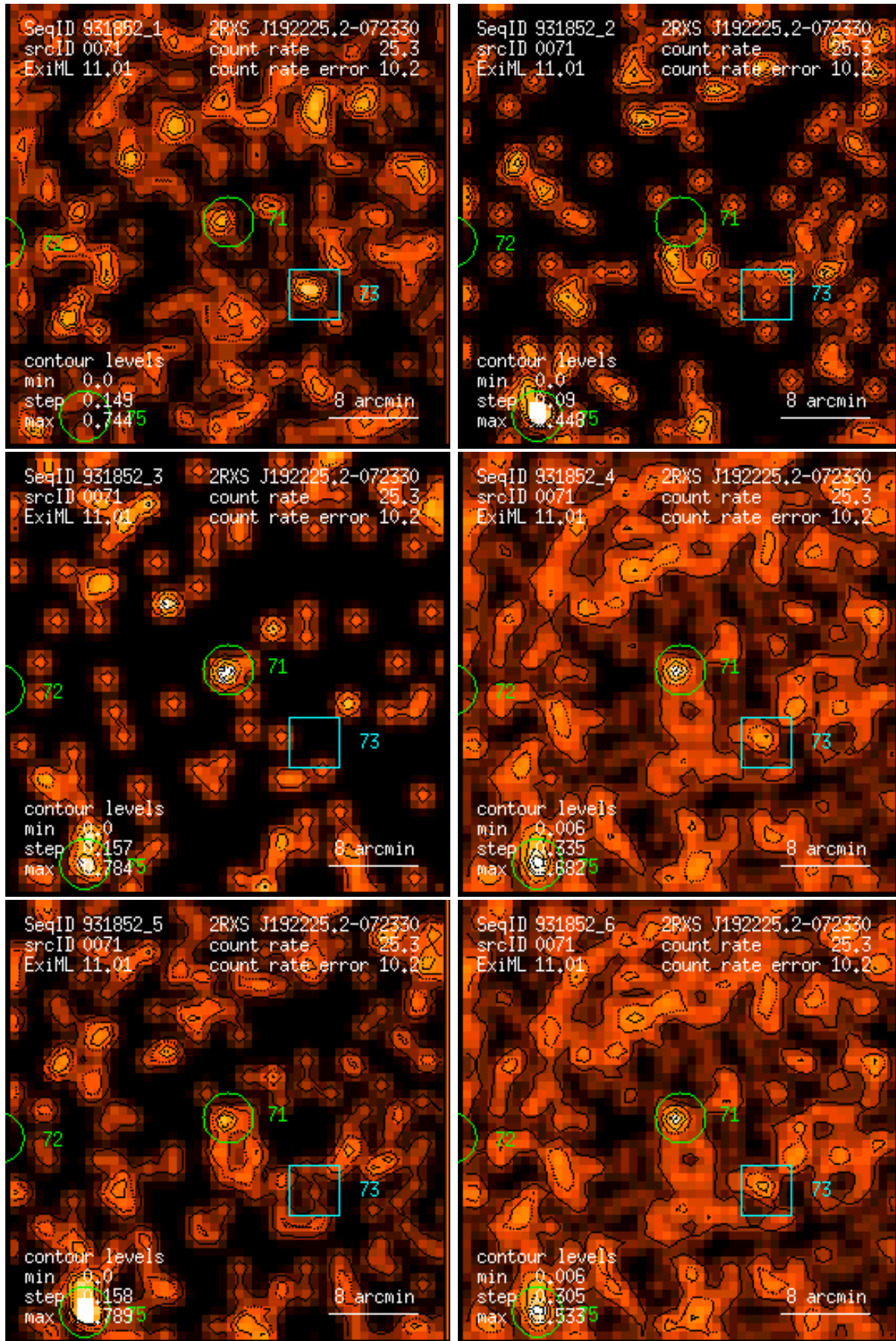
Figure 71: RASS 931852: detection 0071: band rate images, Gaussian filter: (1) PSPC channels 11 – 41, (2) 52 – 90, (3) 91 – 201, (4) 11 – 235, (5) 52 – 201, (6) 11 – 201. Broad band rates in counts/ks. Band rate contour levels in counts/ks/arcmin 2 .
