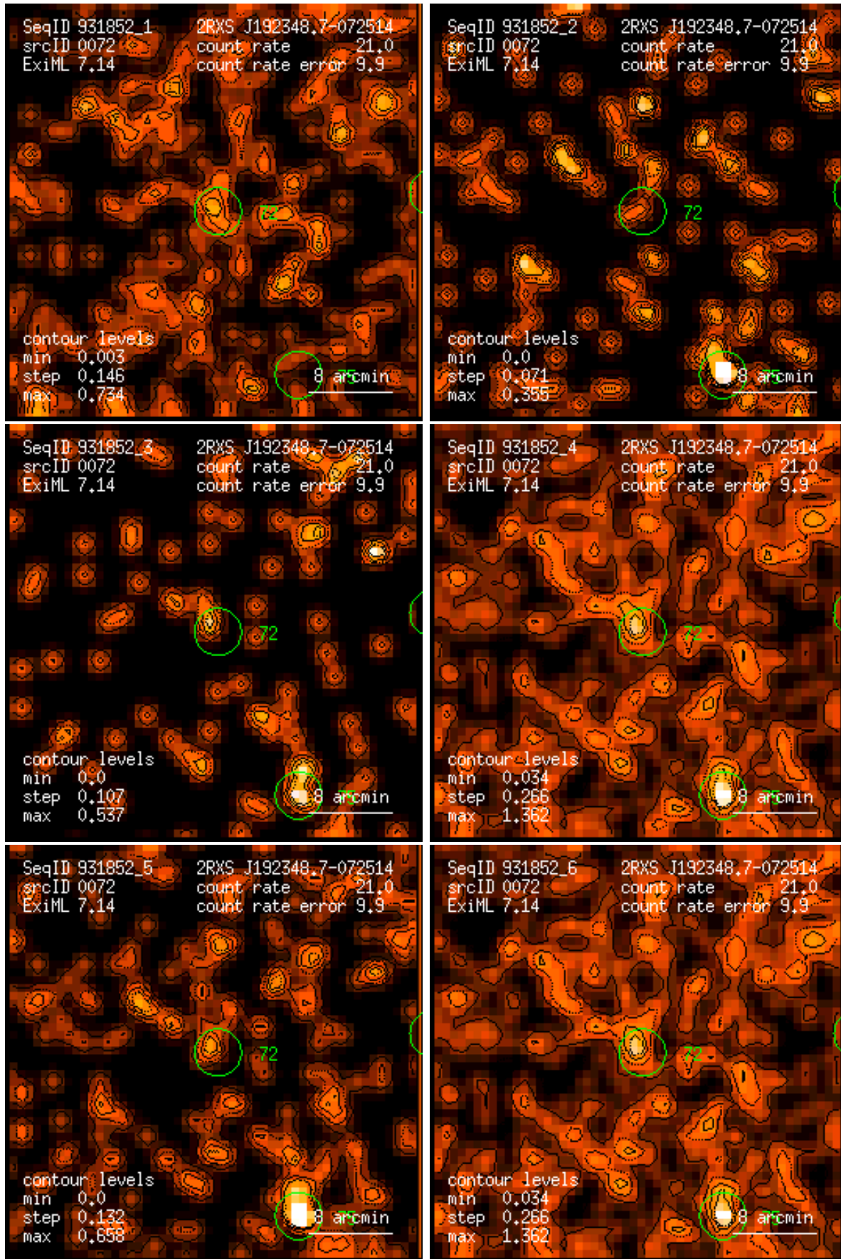
Figure 72: RASS 931852: detection 0072: band rate images, Gaussian filter: (1) PSPC channels 11 – 41, (2) 52 – 90, (3) 91 – 201, (4) 11 – 235, (5) 52 – 201, (6) 11 – 201. Broad band rates in counts/ks. Band rate contour levels in counts/ks/arcmin 2 .
