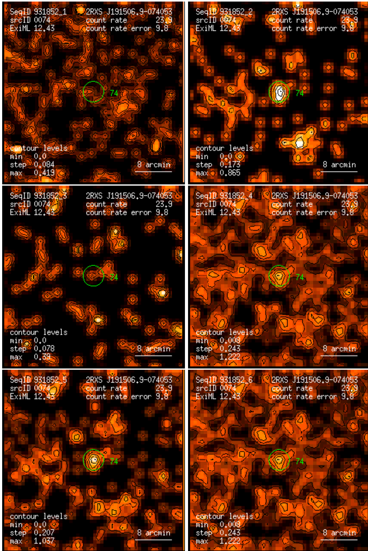
Figure 74: RASS 931852: detection 0074: band rate images, Gaussian filter: (1) PSPC channels 11 – 41, (2) 52 – 90, (3) 91 – 201, (4) 11 – 235, (5) 52 – 201, (6) 11 – 201. Broad band rates in counts/ks. Band rate contour levels in counts/ks/arcmin 2 .
