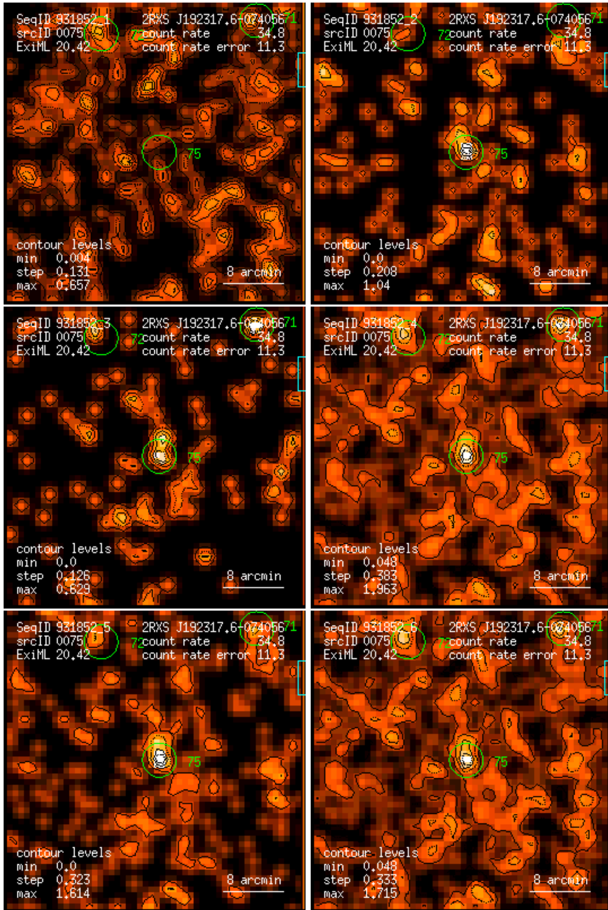
Figure 75: RASS 931852: detection 0075: band rate images, Gaussian filter: (1) PSPC channels 11 – 41, (2) 52 – 90, (3) 91 – 201, (4) 11 – 235, (5) 52 – 201, (6) 11 – 201. Broad band rates in counts/ks. Band rate contour levels in counts/ks/arcmin 2 .
