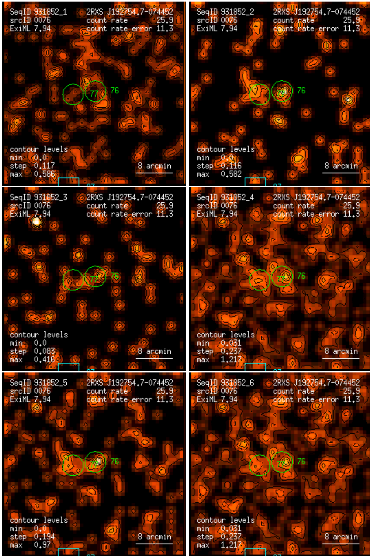
Figure 76: RASS 931852: detection 0076: band rate images, Gaussian filter: (1) PSPC channels 11 – 41, (2) 52 – 90, (3) 91 – 201, (4) 11 – 235, (5) 52 – 201, (6) 11 – 201. Broad band rates in counts/ks. Band rate contour levels in counts/ks/arcmin 2 .
