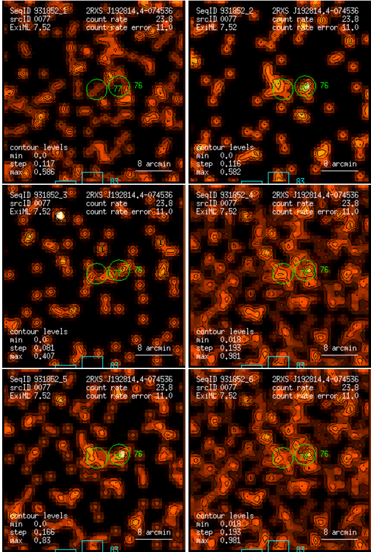
Figure 77: RASS 931852: detection 0077: band rate images, Gaussian filter: (1) PSPC channels 11 – 41, (2) 52 – 90, (3) 91 – 201, (4) 11 – 235, (5) 52 – 201, (6) 11 – 201. Broad band rates in counts/ks. Band rate contour levels in counts/ks/arcmin 2 .
