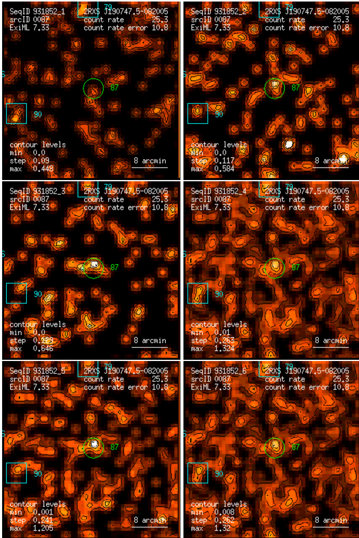
Figure 87: RASS 931852: detection 0087: band rate images, Gaussian filter: (1) PSPC channels 11 – 41, (2) 52 – 90, (3) 91 – 201, (4) 11 – 235, (5) 52 – 201, (6) 11 – 201. Broad band rates in counts/ks. Band rate contour levels in counts/ks/arcmin 2 .
