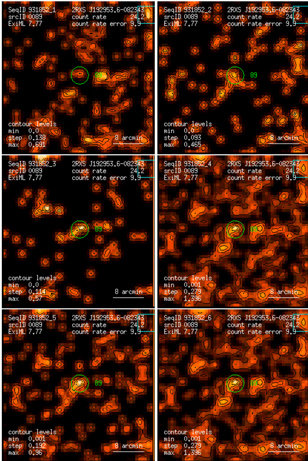
Figure 89: RASS 931852: detection 0089: band rate images, Gaussian filter: (1) PSPC channels 11 – 41, (2) 52 – 90, (3) 91 – 201, (4) 11 – 235, (5) 52 – 201, (6) 11 – 201. Broad band rates in counts/ks. Band rate contour levels in counts/ks/arcmin 2 .
