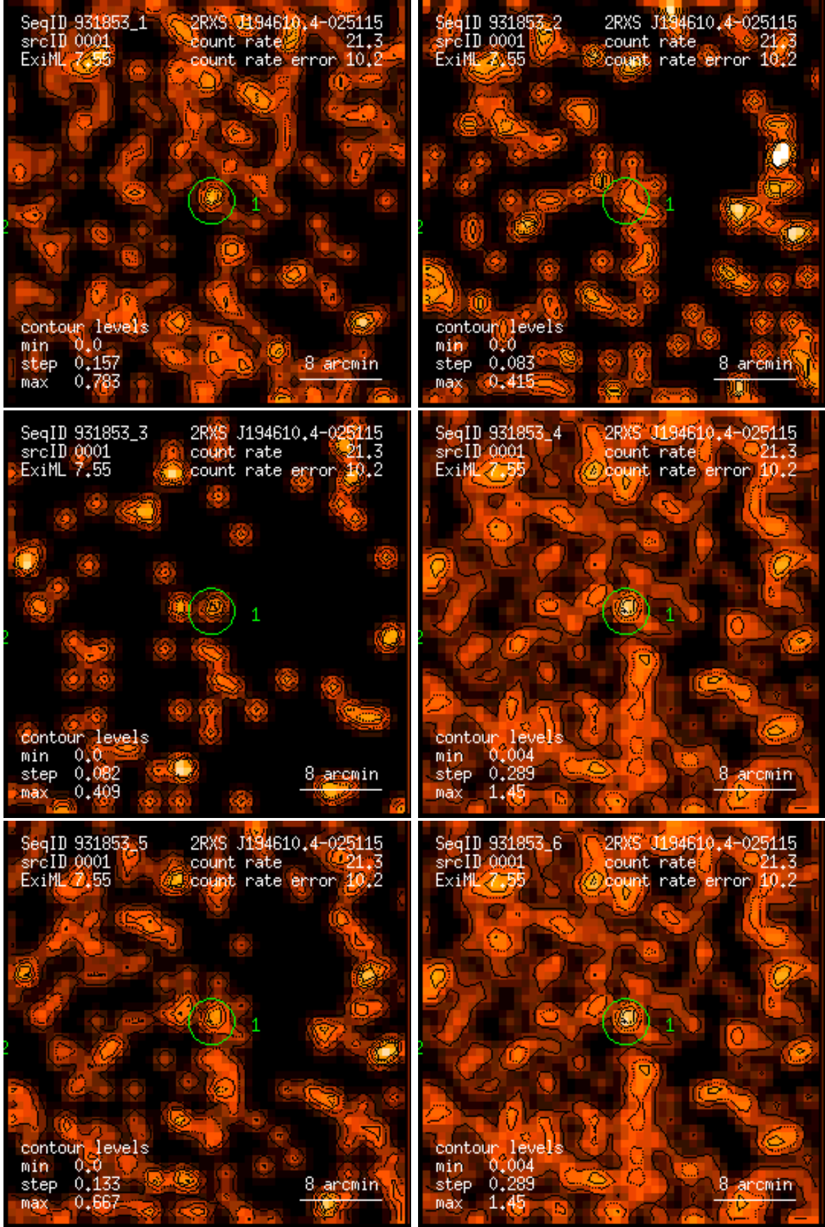
Figure 1: RASS 931853: detection 0001: band rate images, Gaussian filter: (1) PSPC channels 11 – 41, (2) 52 – 90, (3) 91 – 201, (4) 11 – 235, (5) 52 – 201, (6) 11 – 201. Broad band rates in counts/ks. Band rate contour levels in counts/ks/arcmin 2 .
