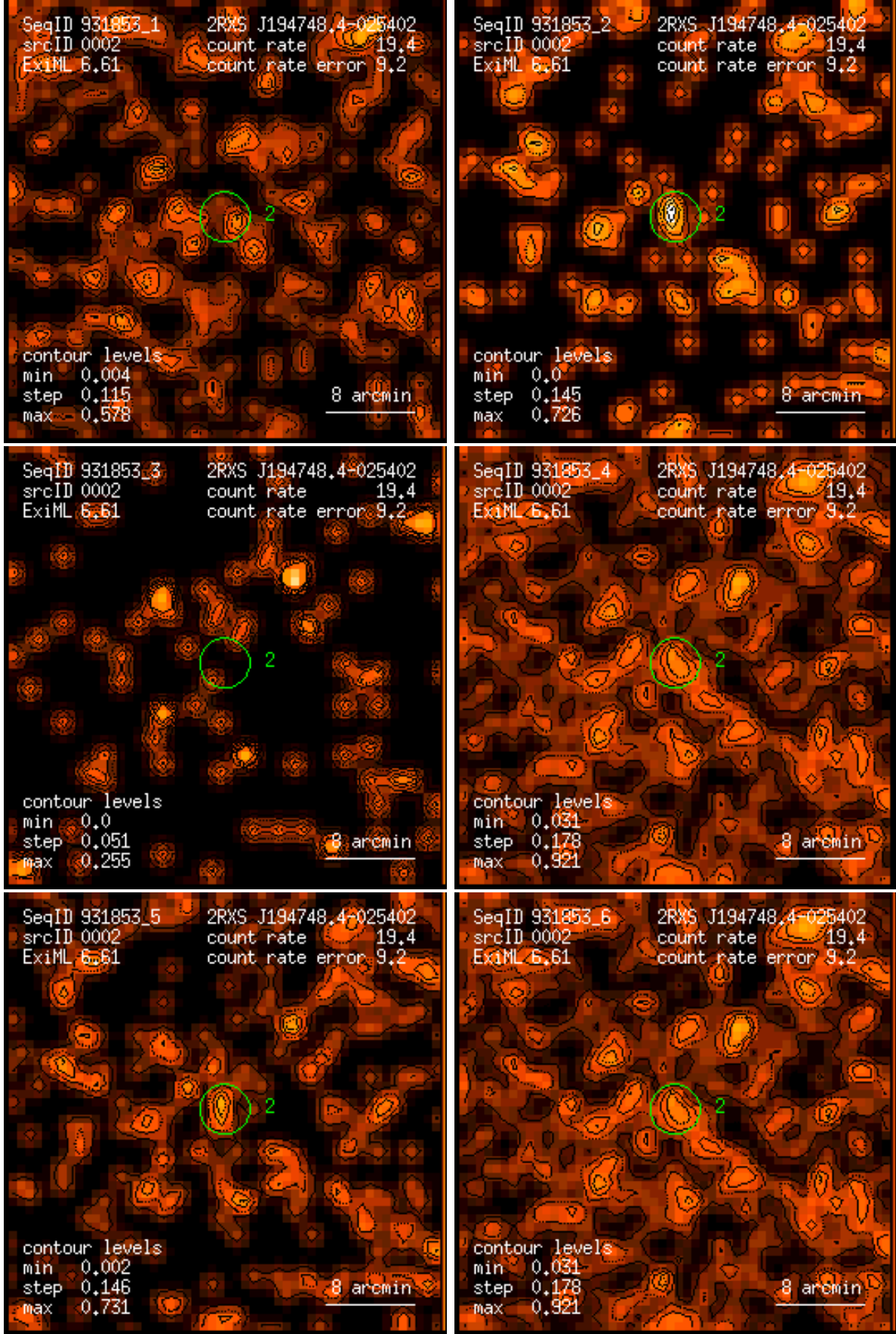
Figure 2: RASS 931853: detection 0002: band rate images, Gaussian filter: (1) PSPC channels 11 – 41, (2) 52 – 90, (3) 91 – 201, (4) 11 – 235, (5) 52 – 201, (6) 11 – 201. Broad band rates in counts/ks. Band rate contour levels in counts/ks/arcmin 2 .
