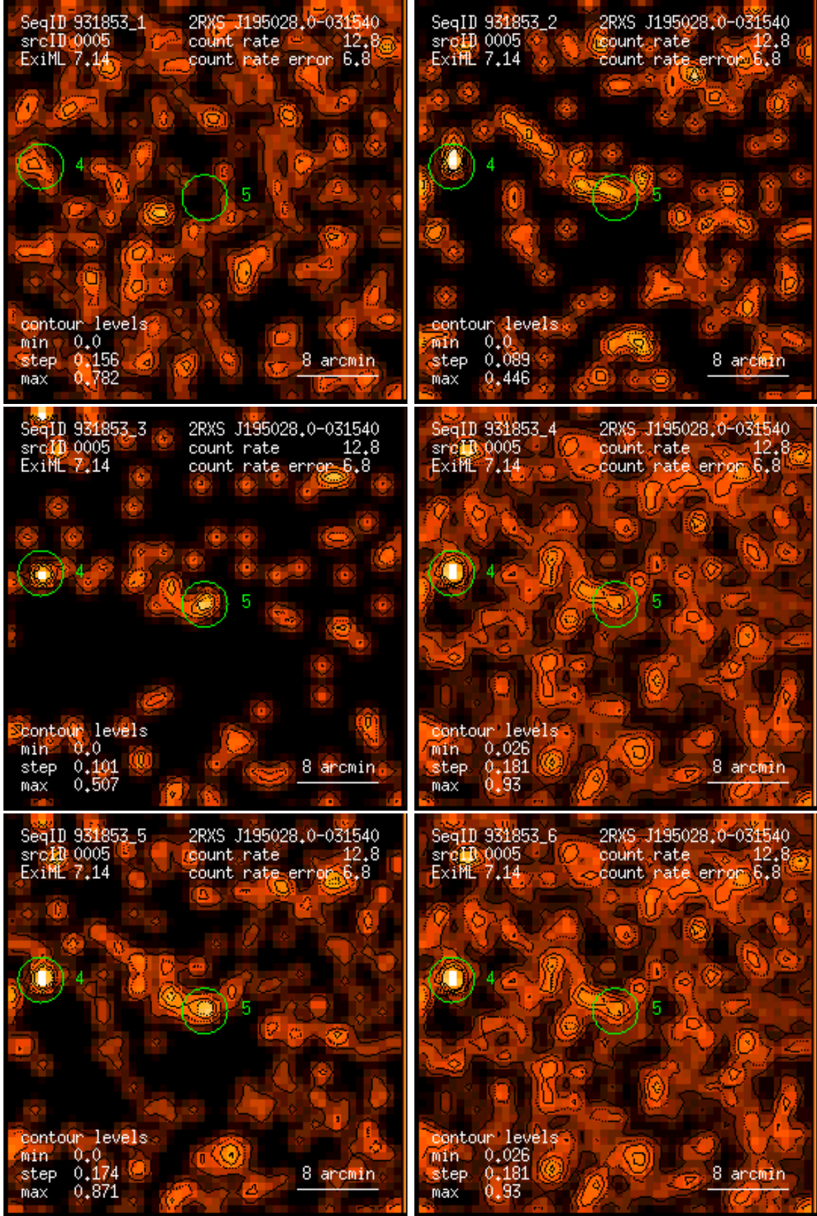
Figure 5: RASS 931853: detection 0005: band rate images, Gaussian filter: (1) PSPC channels 11 – 41, (2) 52 – 90, (3) 91 – 201, (4) 11 – 235, (5) 52 – 201, (6) 11 – 201. Broad band rates in counts/ks. Band rate contour levels in counts/ks/arcmin 2 .
