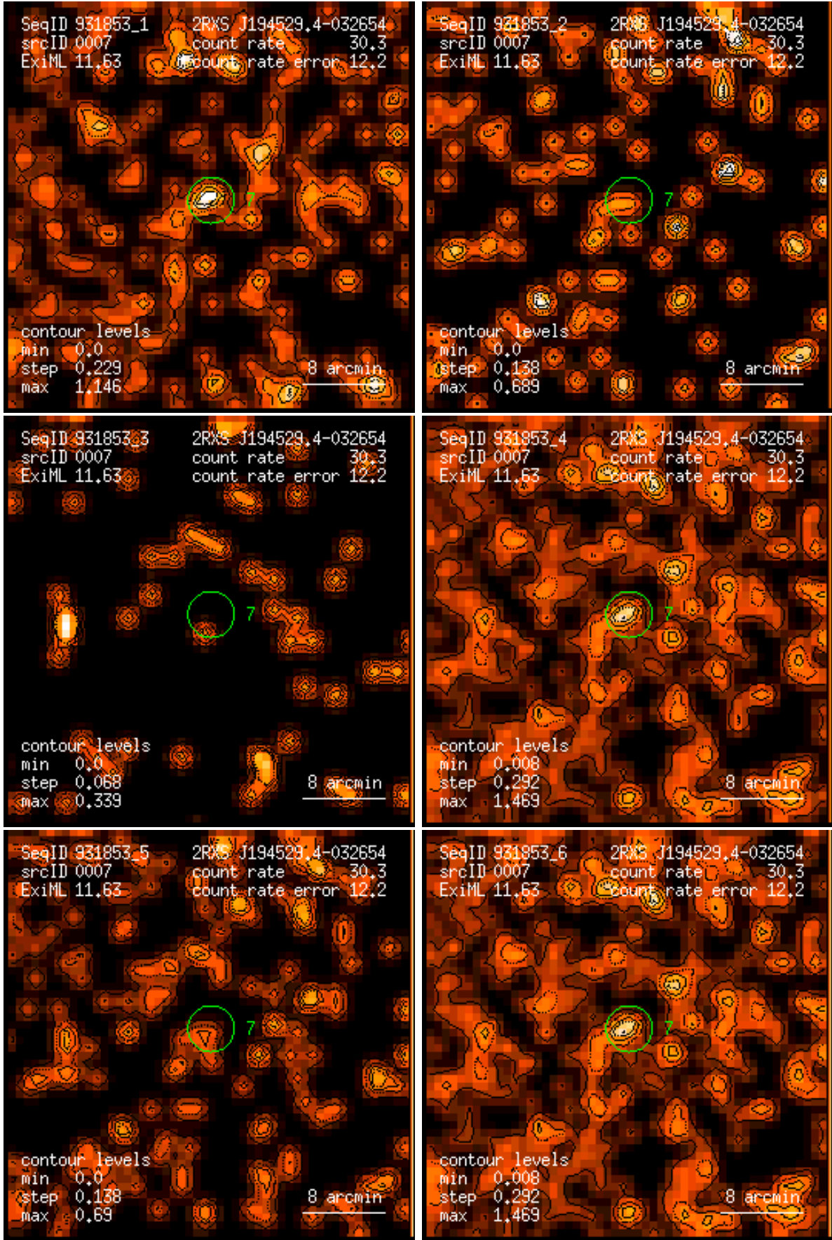
Figure 7: RASS 931853: detection 0007: band rate images, Gaussian filter: (1) PSPC channels 11 – 41, (2) 52 – 90, (3) 91 – 201, (4) 11 – 235, (5) 52 – 201, (6) 11 – 201. Broad band rates in counts/ks. Band rate contour levels in counts/ks/arcmin 2 .
