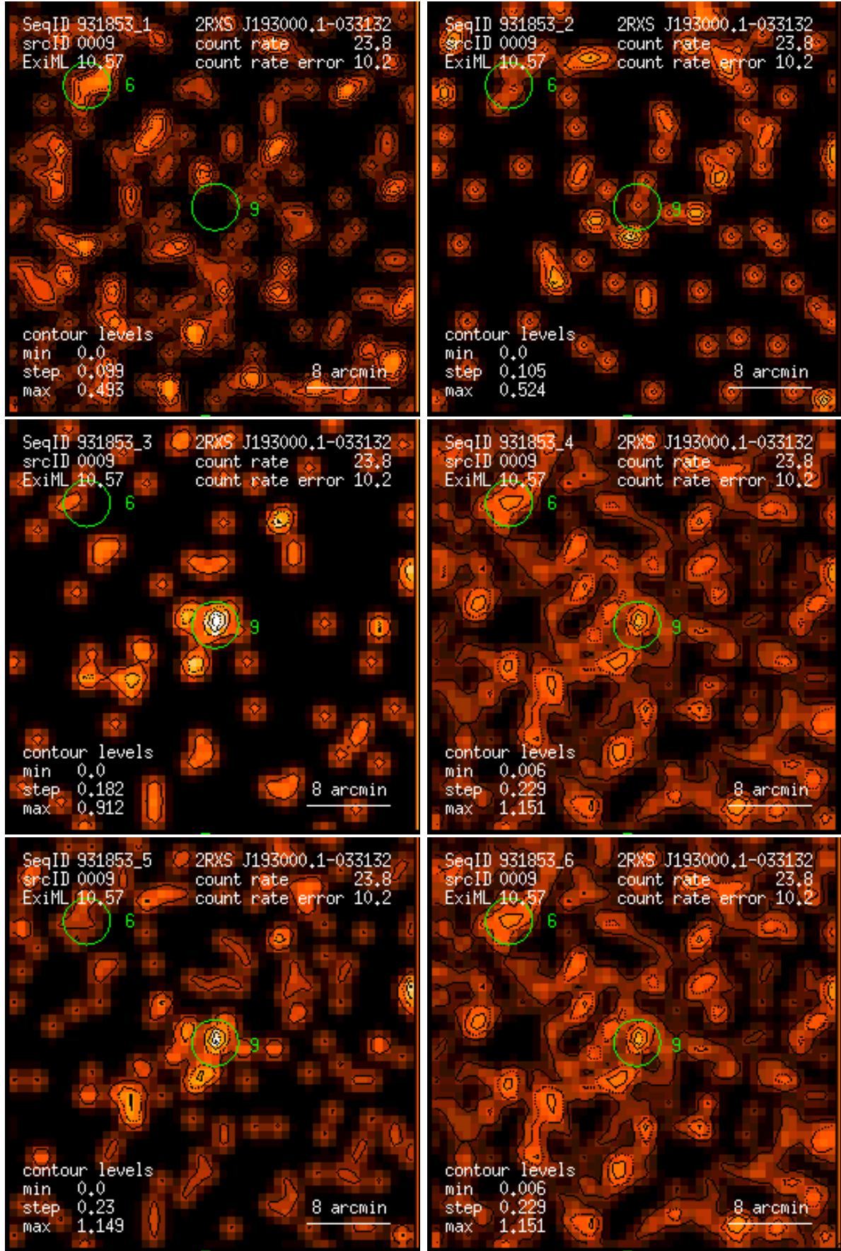
Figure 9: RASS 931853: detection 0009: band rate images, Gaussian filter: (1) PSPC channels 11 – 41, (2) 52 – 90, (3) 91 – 201, (4) 11 – 235, (5) 52 – 201, (6) 11 – 201. Broad band rates in counts/ks. Band rate contour levels in counts/ks/arcmin 2 .
