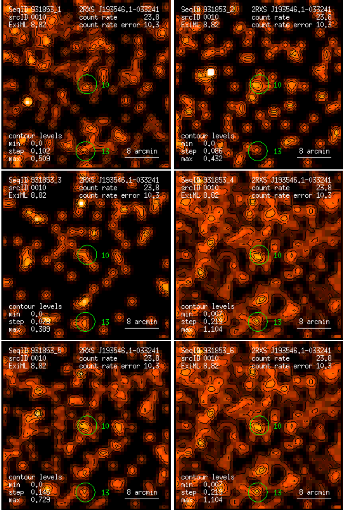
Figure 10: RASS 931853: detection 0010: band rate images, Gaussian filter: (1) PSPC channels 11 – 41, (2) 52 – 90, (3) 91 – 201, (4) 11 – 235, (5) 52 – 201, (6) 11 – 201. Broad band rates in counts/ks. Band rate contour levels in counts/ks/arcmin 2 .
