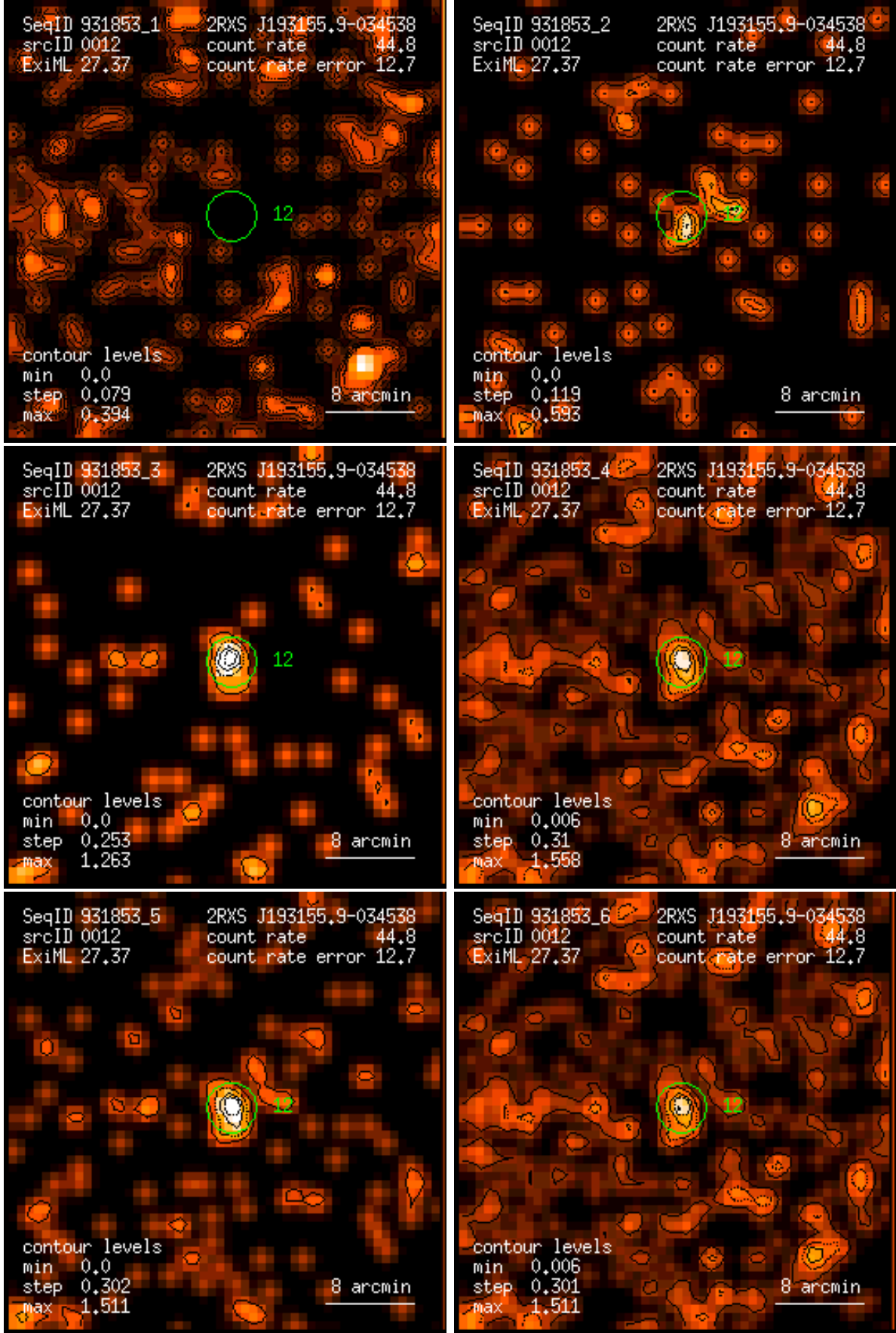
Figure 12: RASS 931853: detection 0012: band rate images, Gaussian filter: (1) PSPC channels 11 – 41, (2) 52 – 90, (3) 91 – 201, (4) 11 – 235, (5) 52 – 201, (6) 11 – 201. Broad band rates in counts/ks. Band rate contour levels in counts/ks/arcmin 2 .
