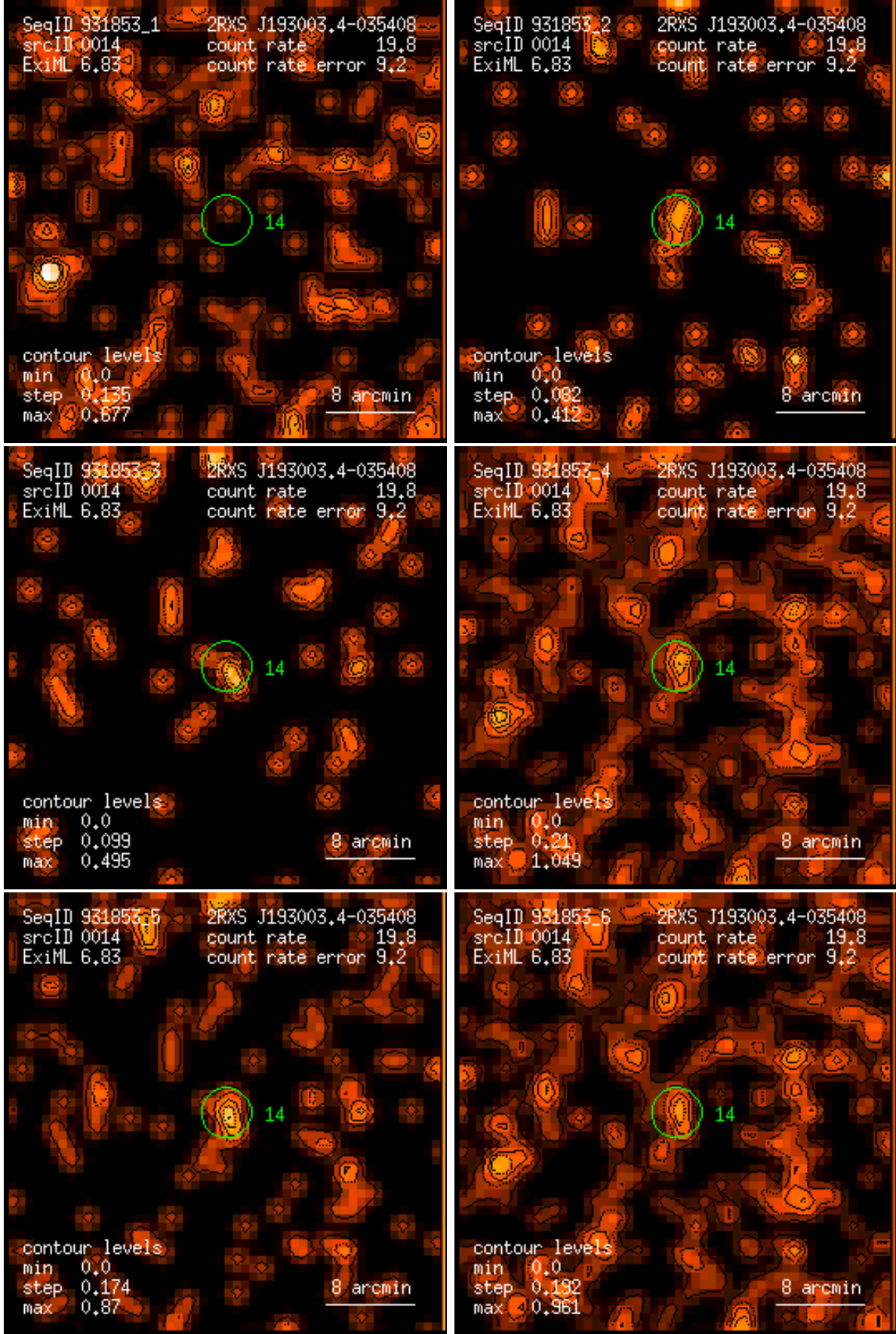
Figure 14: RASS 931853: detection 0014: band rate images, Gaussian filter: (1) PSPC channels 11 – 41, (2) 52 – 90, (3) 91 – 201, (4) 11 – 235, (5) 52 – 201, (6) 11 – 201. Broad band rates in counts/ks. Band rate contour levels in counts/ks/arcmin 2 .
