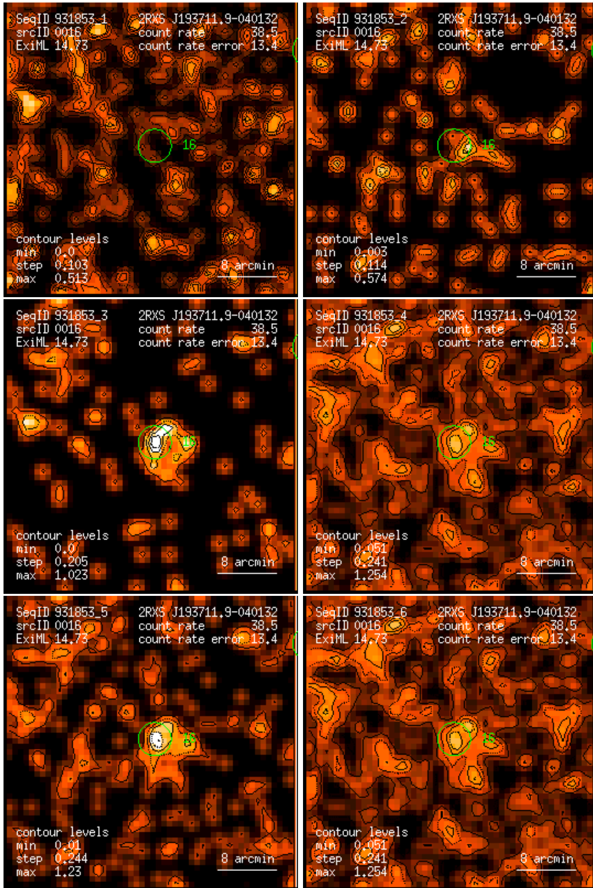
Figure 16: RASS 931853: detection 0016: band rate images, Gaussian filter: (1) PSPC channels 11 – 41, (2) 52 – 90, (3) 91 – 201, (4) 11 – 235, (5) 52 – 201, (6) 11 – 201. Broad band rates in counts/ks. Band rate contour levels in counts/ks/arcmin 2 .
