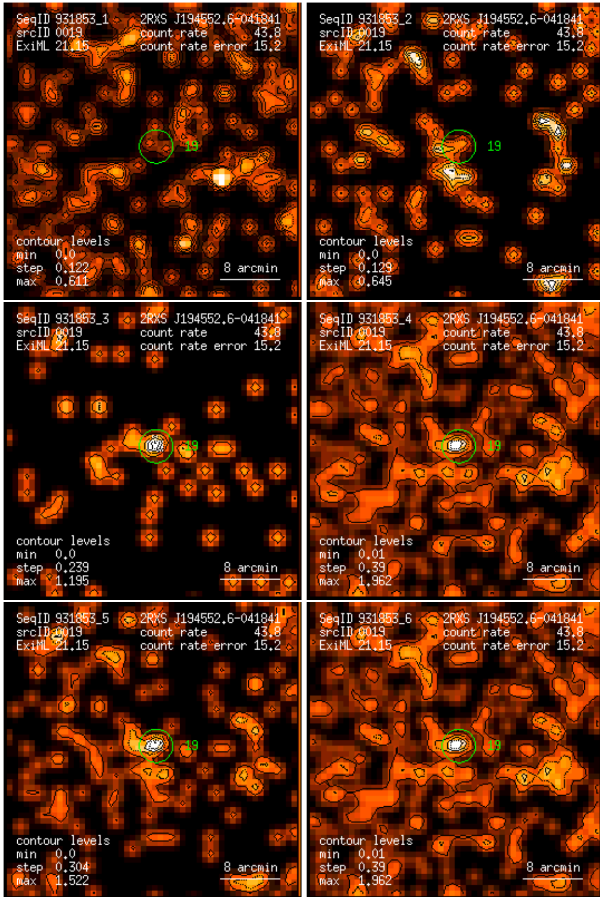
Figure 19: RASS 931853: detection 0019: band rate images, Gaussian filter: (1) PSPC channels 11 – 41, (2) 52 – 90, (3) 91 – 201, (4) 11 – 235, (5) 52 – 201, (6) 11 – 201. Broad band rates in counts/ks. Band rate contour levels in counts/ks/arcmin 2 .
