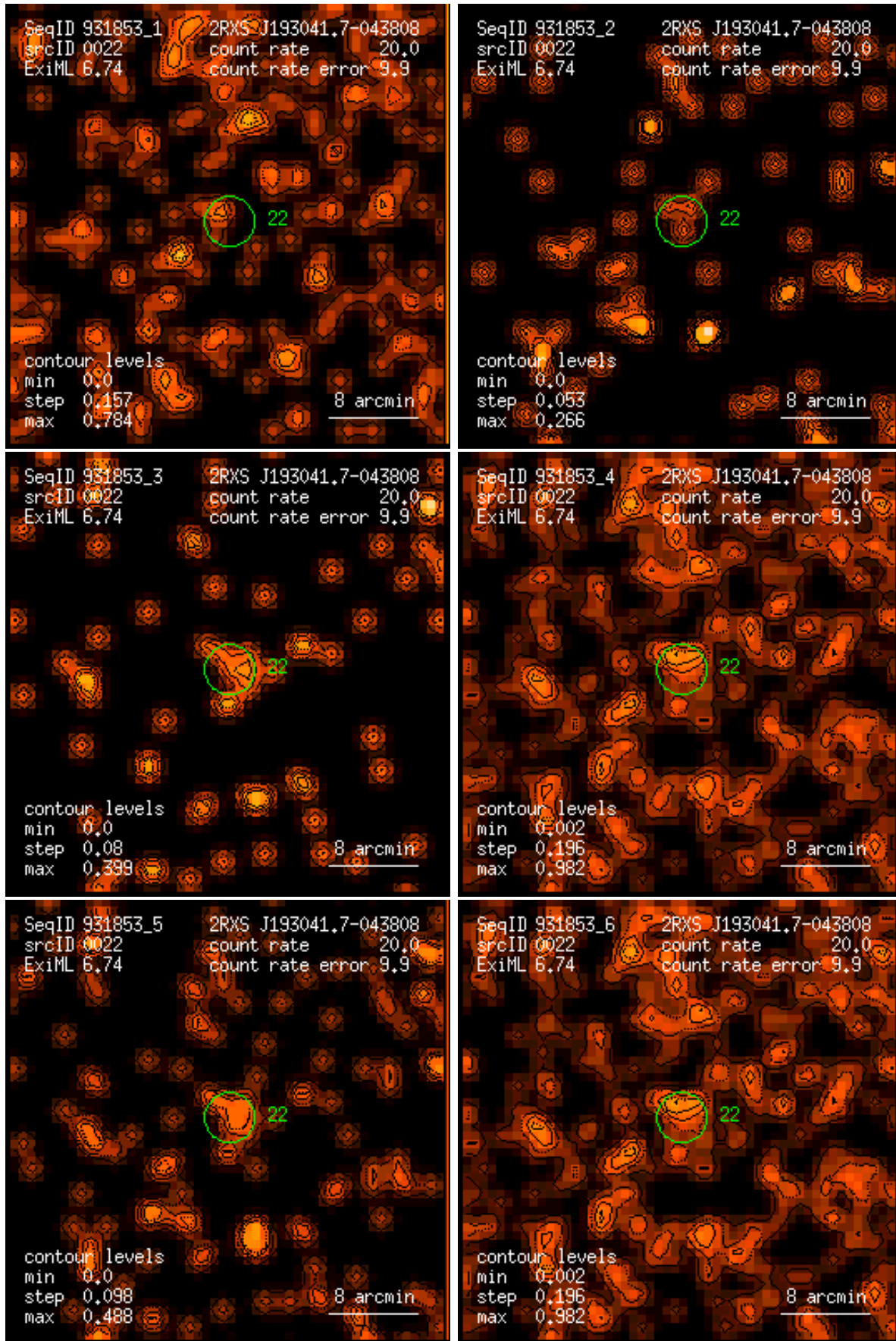
Figure 22: RASS 931853: detection 0022: band rate images, Gaussian filter: (1) PSPC channels 11 – 41, (2) 52 – 90, (3) 91 – 201, (4) 11 – 235, (5) 52 – 201, (6) 11 – 201. Broad band rates in counts/ks. Band rate contour levels in counts/ks/arcmin 2 .
