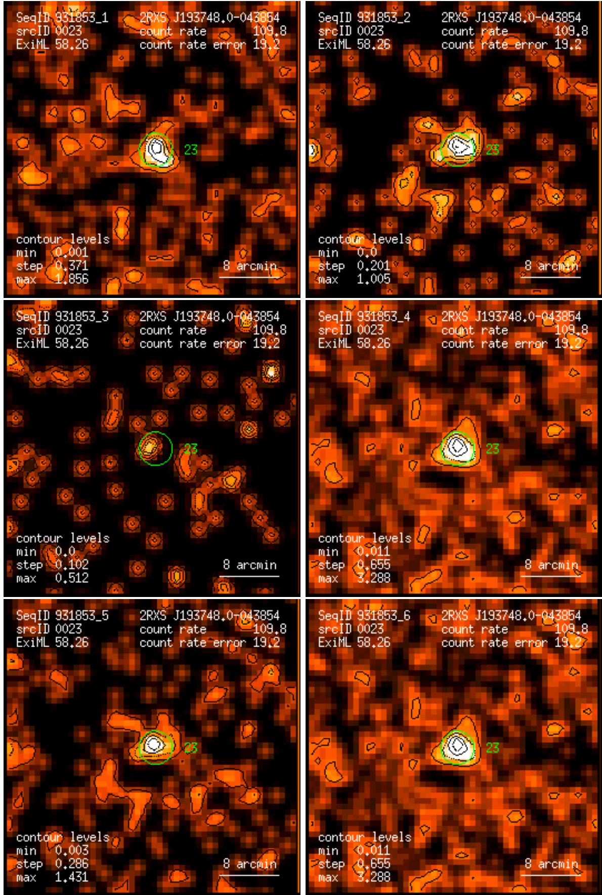
Figure 23: RASS 931853: detection 0023: band rate images, Gaussian filter: (1) PSPC channels 11 – 41, (2) 52 – 90, (3) 91 – 201, (4) 11 – 235, (5) 52 – 201, (6) 11 – 201. Broad band rates in counts/ks. Band rate contour levels in counts/ks/arcmin 2 .
