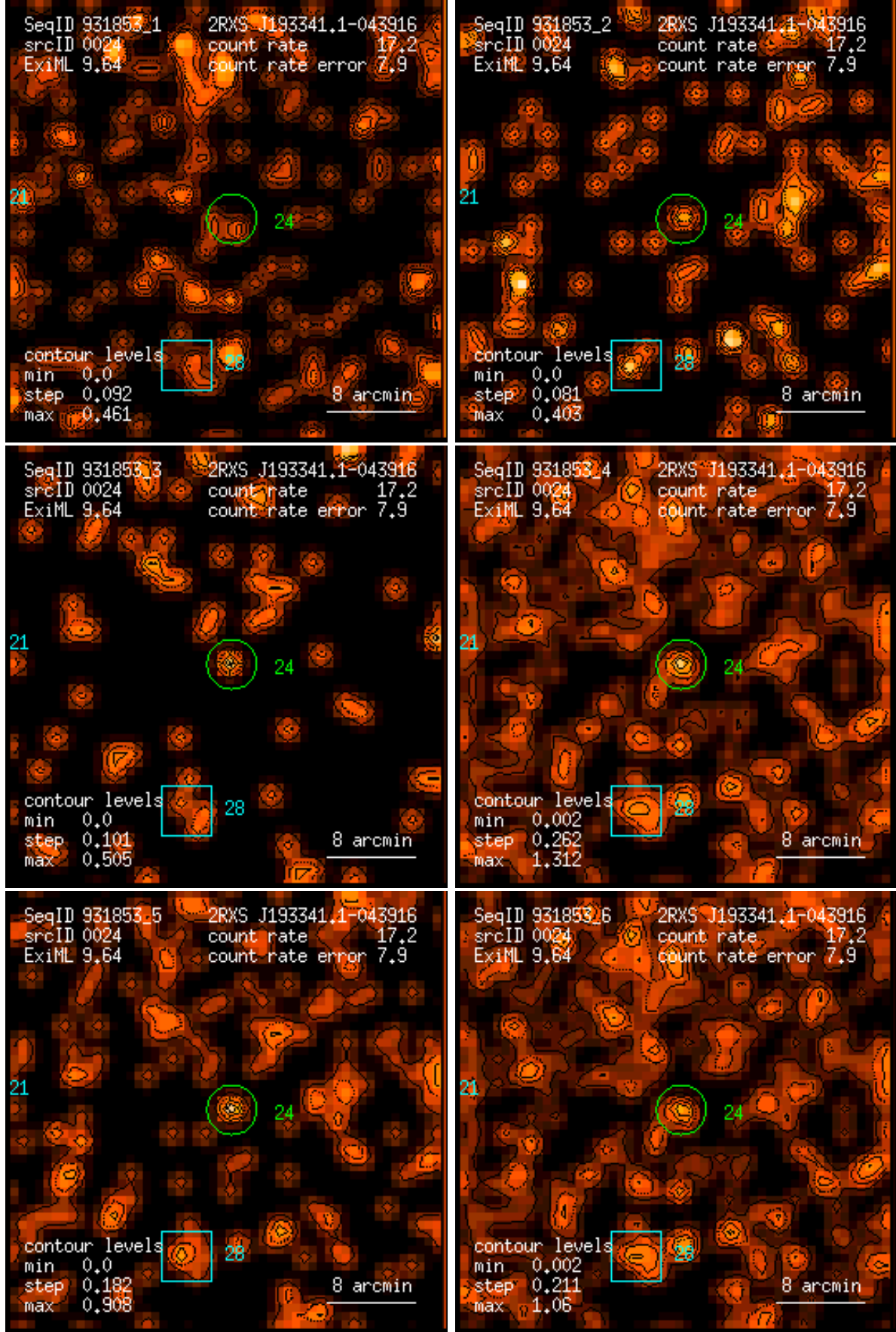
Figure 24: RASS 931853: detection 0024: band rate images, Gaussian filter: (1) PSPC channels 11 – 41, (2) 52 – 90, (3) 91 – 201, (4) 11 – 235, (5) 52 – 201, (6) 11 – 201. Broad band rates in counts/ks. Band rate contour levels in counts/ks/arcmin 2 .
