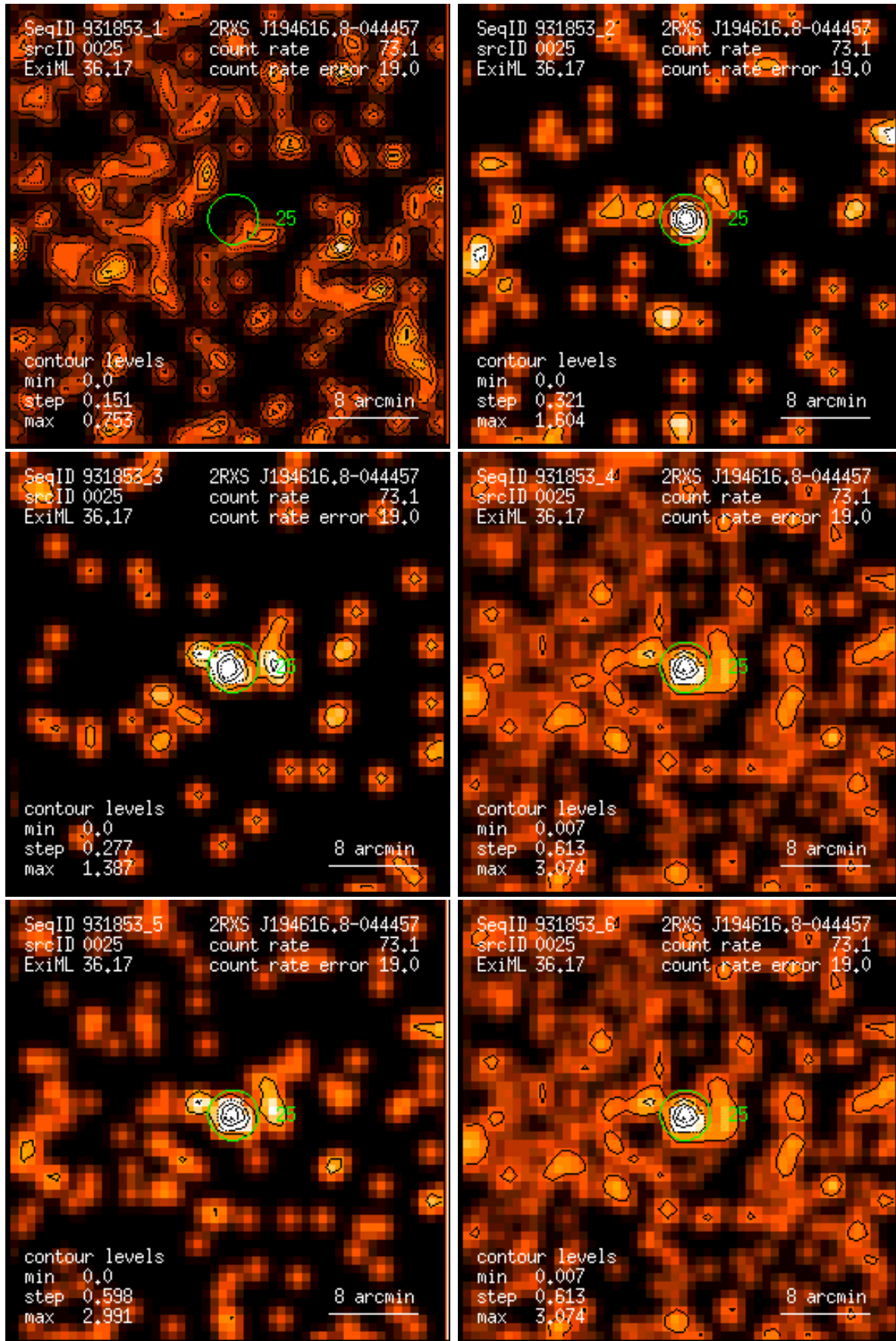
Figure 25: RASS 931853: detection 0025: band rate images, Gaussian filter: (1) PSPC channels 11 – 41, (2) 52 – 90, (3) 91 – 201, (4) 11 – 235, (5) 52 – 201, (6) 11 – 201. Broad band rates in counts/ks. Band rate contour levels in counts/ks/arcmin 2 .
