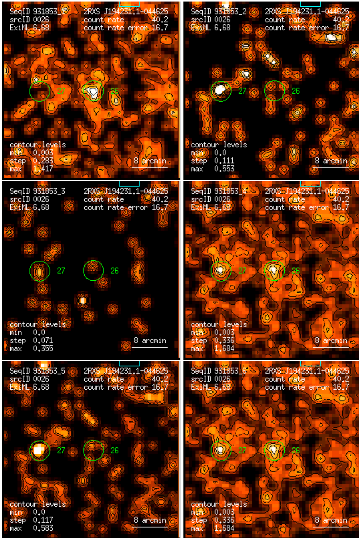
Figure 26: RASS 931853: detection 0026: band rate images, Gaussian filter: (1) PSPC channels 11 – 41, (2) 52 – 90, (3) 91 – 201, (4) 11 – 235, (5) 52 – 201, (6) 11 – 201. Broad band rates in counts/ks. Band rate contour levels in counts/ks/arcmin 2 .
