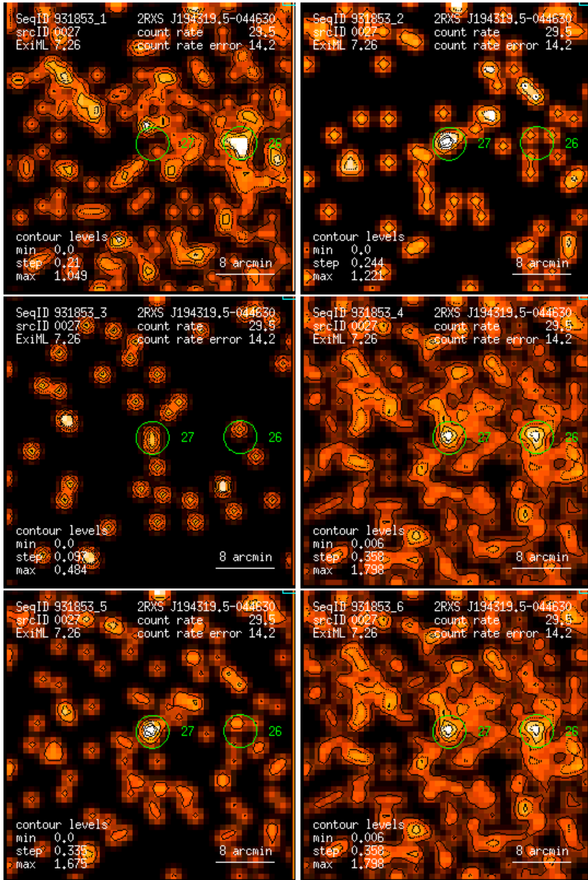
Figure 27: RASS 931853: detection 0027: band rate images, Gaussian filter: (1) PSPC channels 11 – 41, (2) 52 – 90, (3) 91 – 201, (4) 11 – 235, (5) 52 – 201, (6) 11 – 201. Broad band rates in counts/ks. Band rate contour levels in counts/ks/arcmin 2 .
