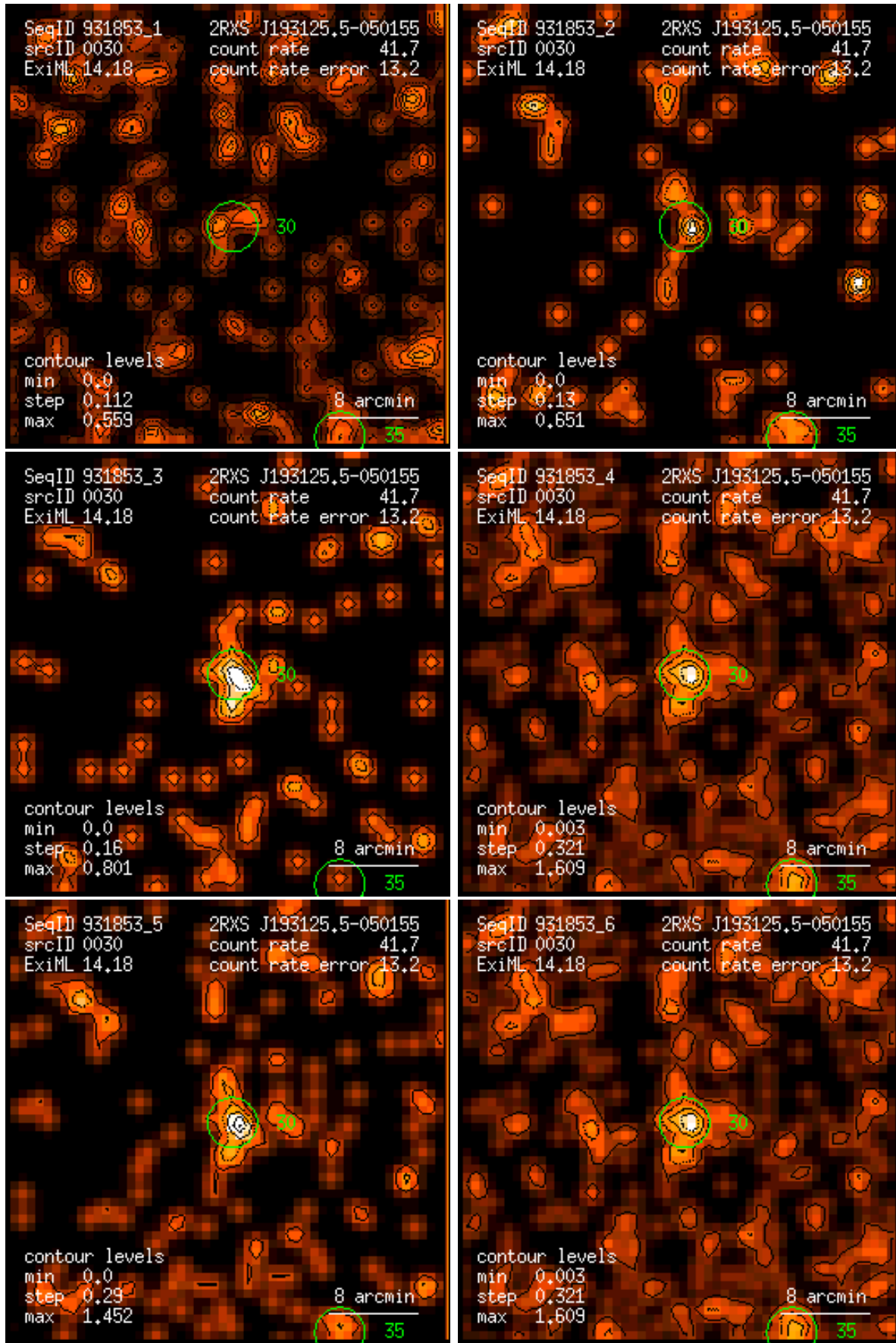
Figure 30: RASS 931853: detection 0030: band rate images, Gaussian filter: (1) PSPC channels 11 – 41, (2) 52 – 90, (3) 91 – 201, (4) 11 – 235, (5) 52 – 201, (6) 11 – 201. Broad band rates in counts/ks. Band rate contour levels in counts/ks/arcmin 2 .
