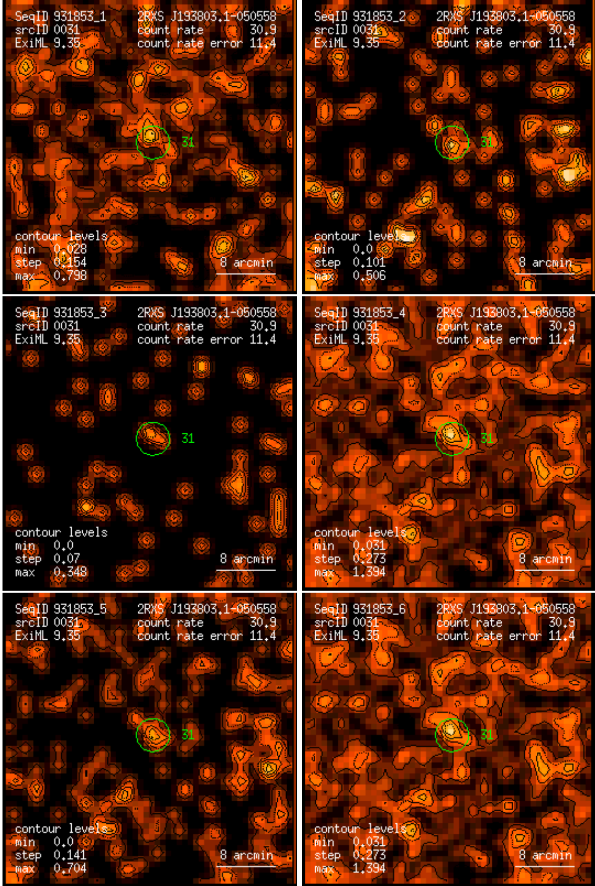
Figure 31: RASS 931853: detection 0031: band rate images, Gaussian filter: (1) PSPC channels 11 – 41, (2) 52 – 90, (3) 91 – 201, (4) 11 – 235, (5) 52 – 201, (6) 11 – 201. Broad band rates in counts/ks. Band rate contour levels in counts/ks/arcmin 2 .
