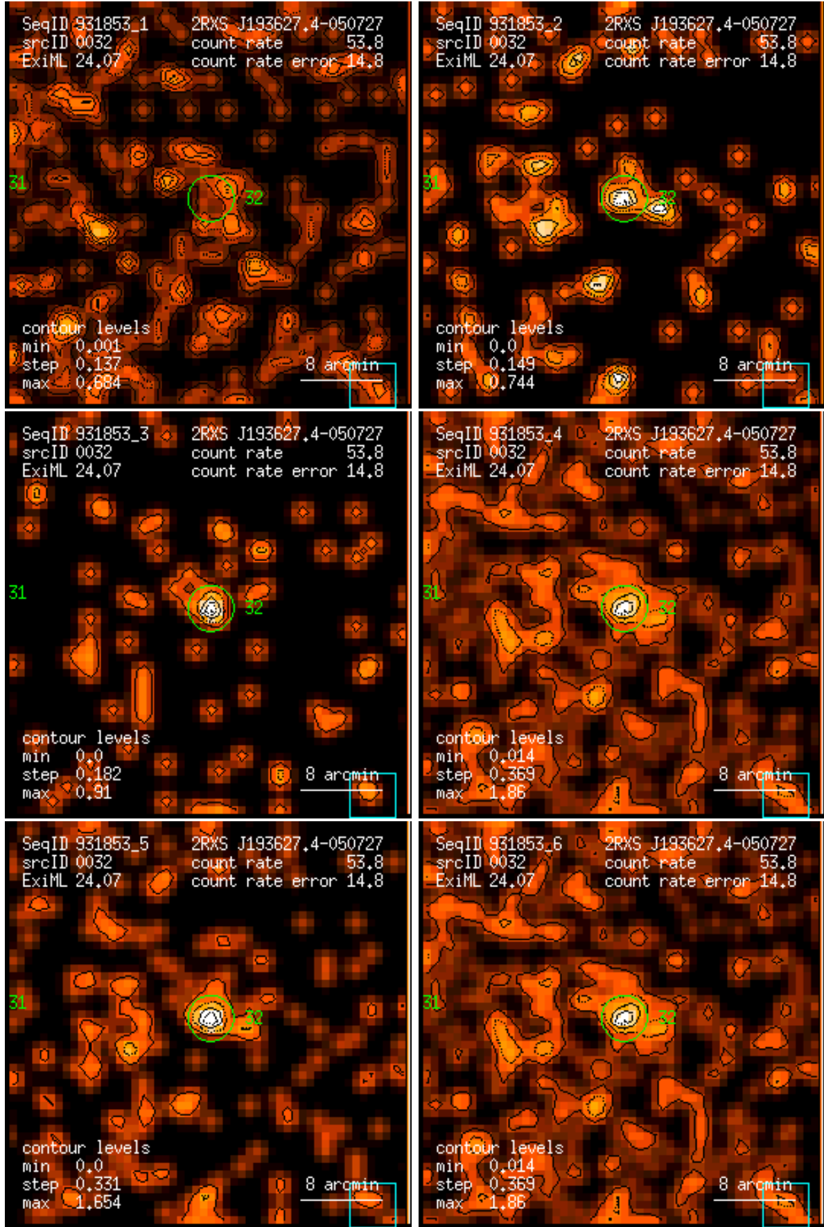
Figure 32: RASS 931853: detection 0032: band rate images, Gaussian filter: (1) PSPC channels 11 – 41, (2) 52 – 90, (3) 91 – 201, (4) 11 – 235, (5) 52 – 201, (6) 11 – 201. Broad band rates in counts/ks. Band rate contour levels in counts/ks/arcmin 2 .
