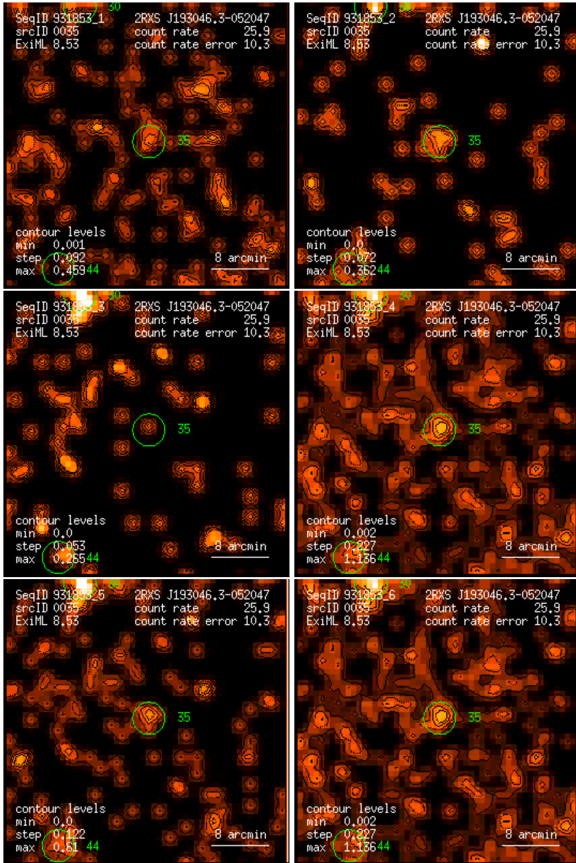
Figure 35: RASS 931853: detection 0035: band rate images, Gaussian filter: (1) PSPC channels 11 – 41, (2) 52 – 90, (3) 91 – 201, (4) 11 – 235, (5) 52 – 201, (6) 11 – 201. Broad band rates in counts/ks. Band rate contour levels in counts/ks/arcmin 2 .
