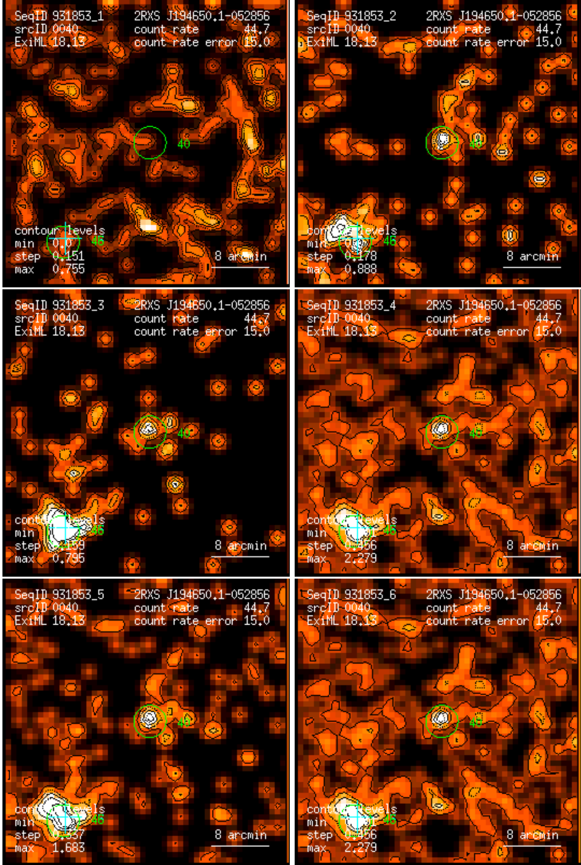
Figure 40: RASS 931853: detection 0040: band rate images, Gaussian filter: (1) PSPC channels 11 – 41, (2) 52 – 90, (3) 91 – 201, (4) 11 – 235, (5) 52 – 201, (6) 11 – 201. Broad band rates in counts/ks. Band rate contour levels in counts/ks/arcmin 2 .
