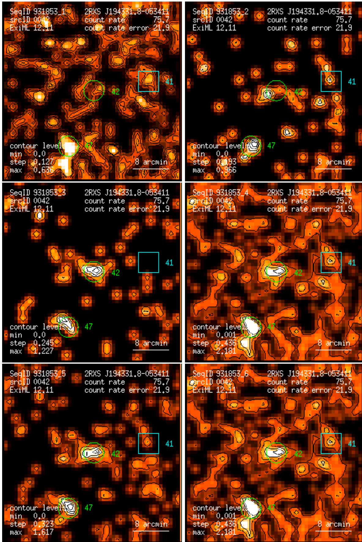
Figure 42: RASS 931853: detection 0042: band rate images, Gaussian filter: (1) PSPC channels 11 – 41, (2) 52 – 90, (3) 91 – 201, (4) 11 – 235, (5) 52 – 201, (6) 11 – 201. Broad band rates in counts/ks. Band rate contour levels in counts/ks/arcmin 2 .
