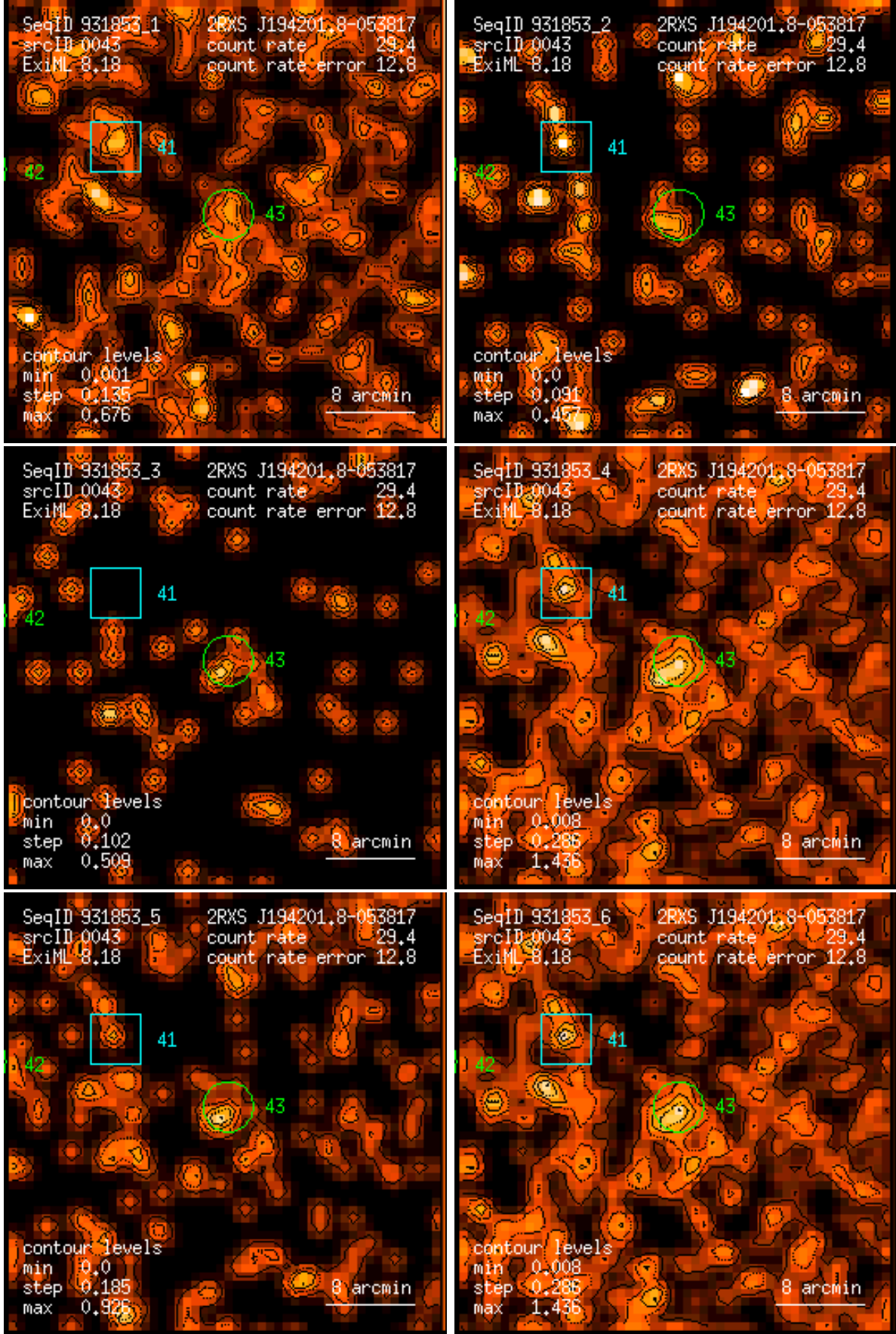
Figure 43: RASS 931853: detection 0043: band rate images, Gaussian filter: (1) PSPC channels 11 – 41, (2) 52 – 90, (3) 91 – 201, (4) 11 – 235, (5) 52 – 201, (6) 11 – 201. Broad band rates in counts/ks. Band rate contour levels in counts/ks/arcmin 2 .
