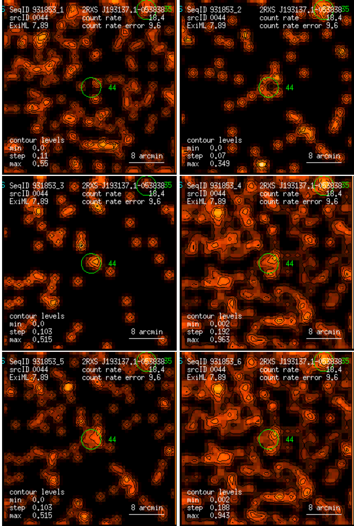
Figure 44: RASS 931853: detection 0044: band rate images, Gaussian filter: (1) PSPC channels 11 – 41, (2) 52 – 90, (3) 91 – 201, (4) 11 – 235, (5) 52 – 201, (6) 11 – 201. Broad band rates in counts/ks. Band rate contour levels in counts/ks/arcmin 2 .
