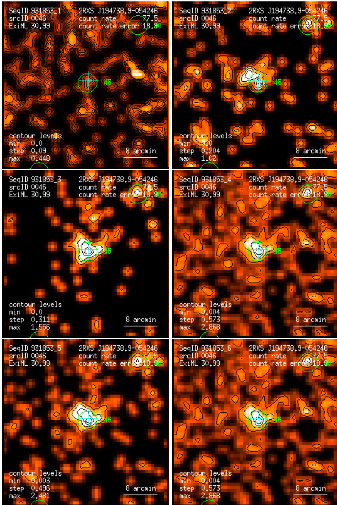
Figure 46: RASS 931853: detection 0046: band rate images, Gaussian filter: (1) PSPC channels 11 – 41, (2) 52 – 90, (3) 91 – 201, (4) 11 – 235, (5) 52 – 201, (6) 11 – 201. Broad band rates in counts/ks. Band rate contour levels in counts/ks/arcmin 2 .
