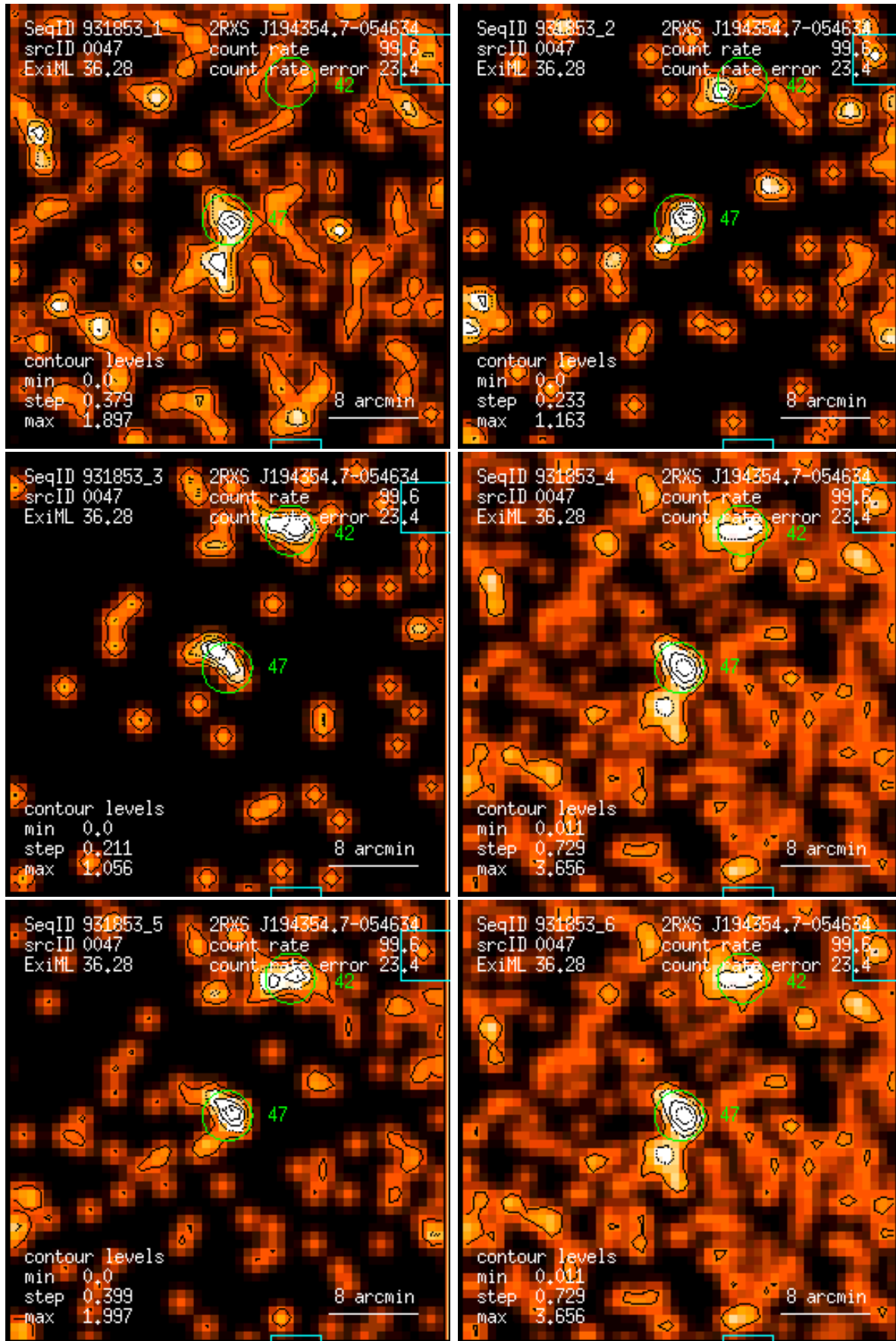
Figure 47: RASS 931853: detection 0047: band rate images, Gaussian filter: (1) PSPC channels 11 – 41, (2) 52 – 90, (3) 91 – 201, (4) 11 – 235, (5) 52 – 201, (6) 11 – 201. Broad band rates in counts/ks. Band rate contour levels in counts/ks/arcmin 2 .
