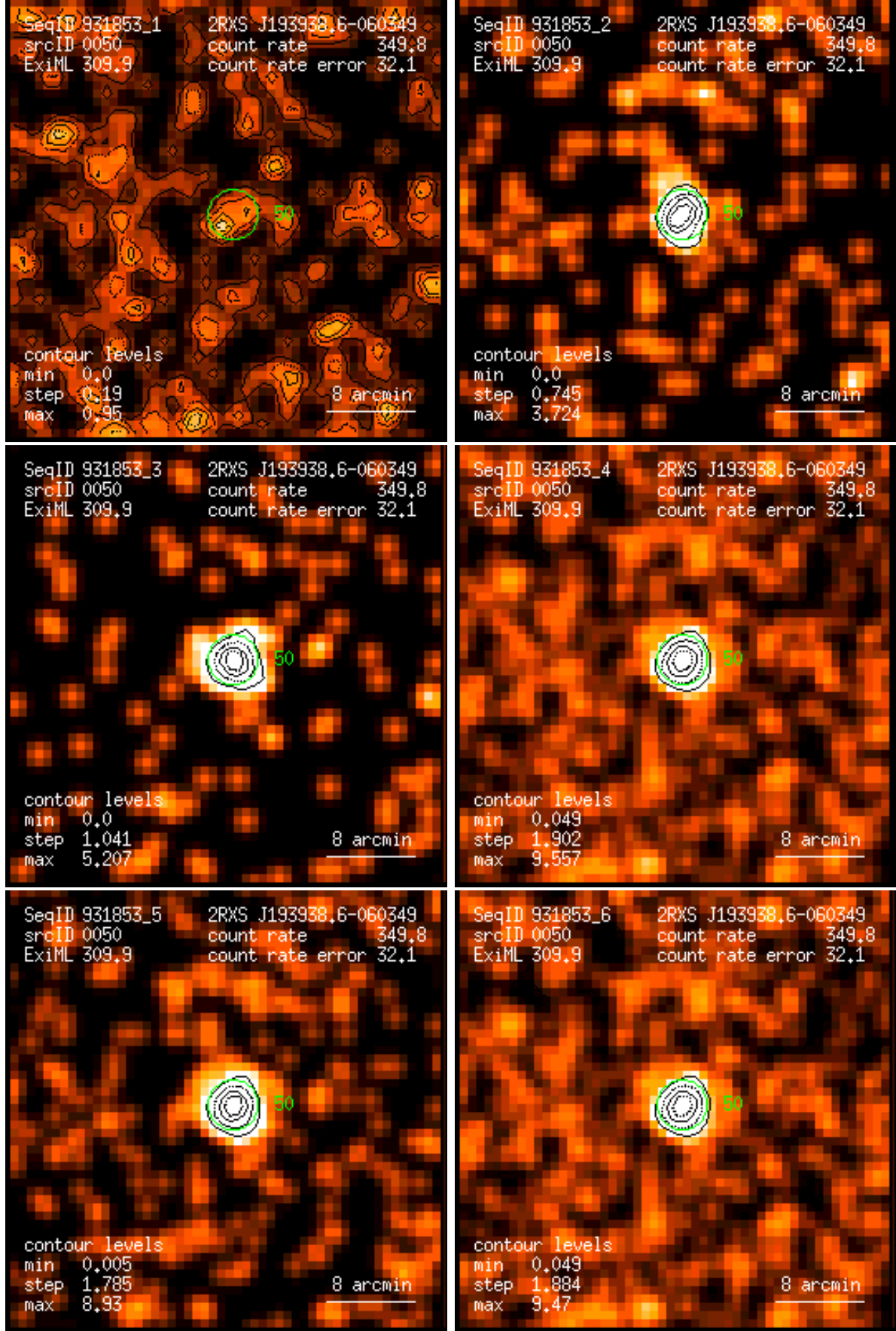
Figure 50: RASS 931853: detection 0050: band rate images, Gaussian filter: (1) PSPC channels 11 – 41, (2) 52 – 90, (3) 91 – 201, (4) 11 – 235, (5) 52 – 201, (6) 11 – 201. Broad band rates in counts/ks. Band rate contour levels in counts/ks/arcmin 2 .
