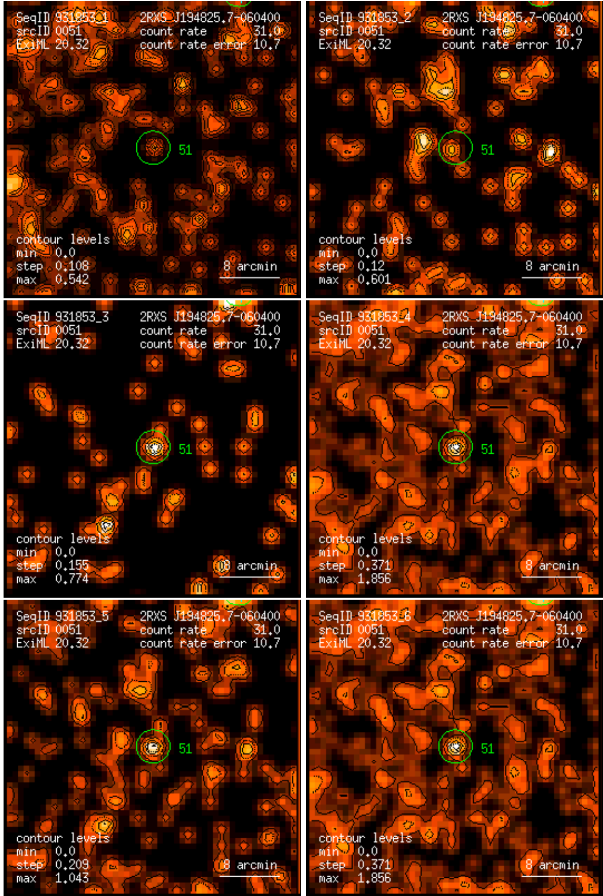
Figure 51: RASS 931853: detection 0051: band rate images, Gaussian filter: (1) PSPC channels 11 – 41, (2) 52 – 90, (3) 91 – 201, (4) 11 – 235, (5) 52 – 201, (6) 11 – 201. Broad band rates in counts/ks. Band rate contour levels in counts/ks/arcmin 2 .
